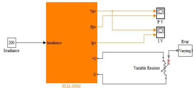
Fig. 5. Simulink characteristic measuring model of solar module
