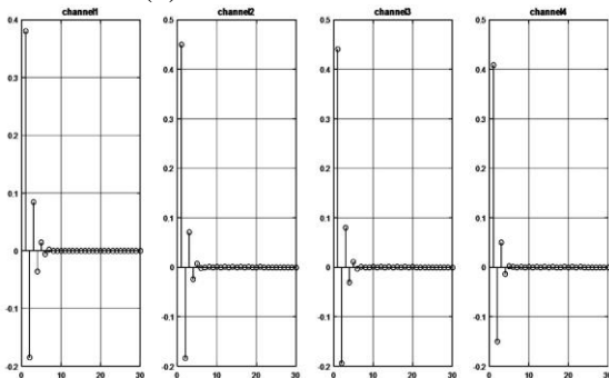
Fig. 3. AAA channel impulse characteristics view
