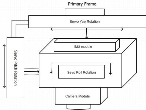
Fig. 1. Primary frame of the imitation stand
