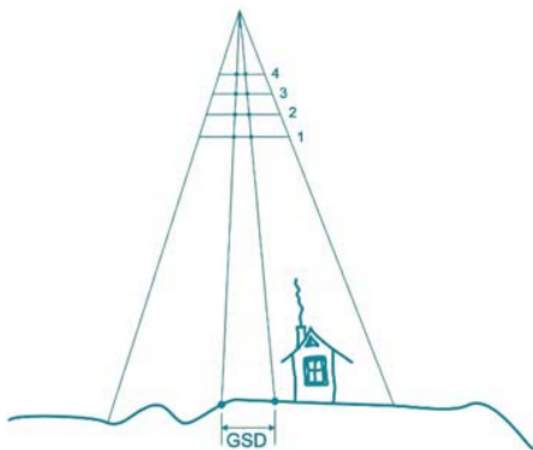
Fig. 6. An example of shooting cameras with different sizes of matrices and GSD
