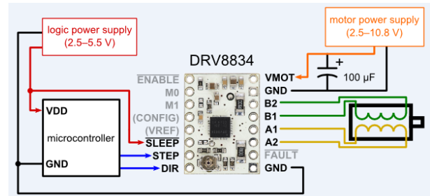
Fig. 3. The electrical wiring diagram
