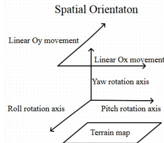
Fig. 4. Spatial movement of the stand
