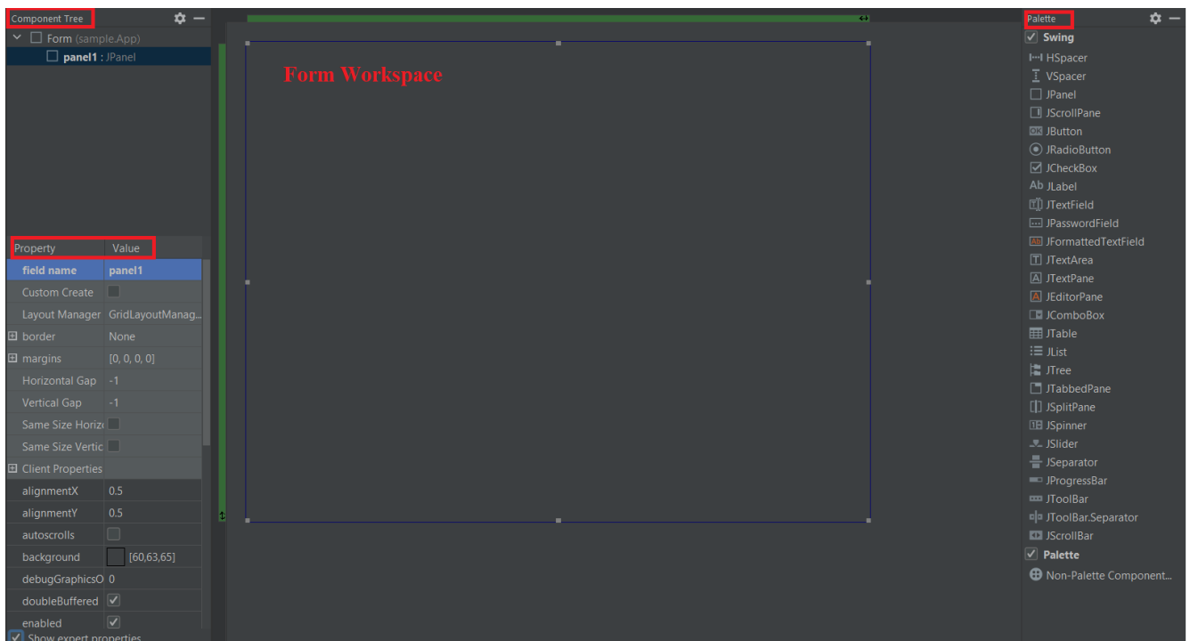
Рис. 2.5. GUI Designer
