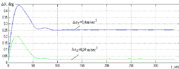
Fig. 4. Effect of measurement errors on the acceleration error calculating the pitch angle
