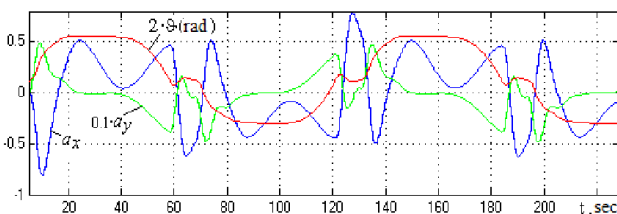
Fig. 5. The change in parameters of longitudinal motion during maneuvering to climb and descent
