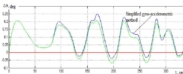
Fig. 9. The errors of pitch measurement by simplified and full algorithms
