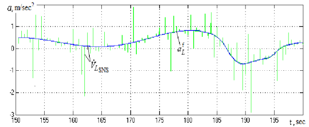
Fig. 2. The estimation results of acceleration a_L^f in comparison with differentiated signal V_{L_{SNS}} during the UAV maneuver "Zoom"
