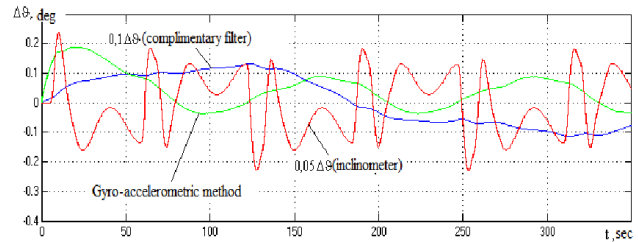
Fig. 6. Pitch errors measurement using different measuring sensors
