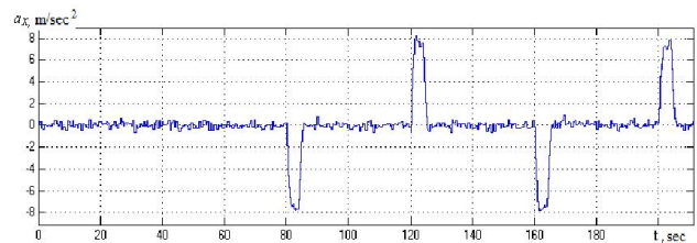
Fig. 7. Acceleration acting on the UAV with highly energetic maneuvering (climbing and descending)
