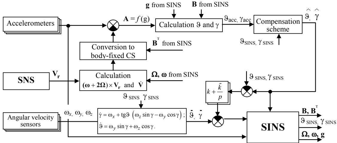
Fig. 1. The block diagram of scheme to measure the angular orientation by gyro-accelerometric method
