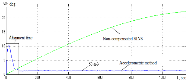
Fig. 3. The illustration of the change of pitch measurement errors with no maneuvering
