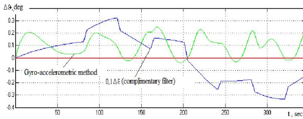
Fig. 8. The change in errors of measuring during energetic maneuvering with the climbing and descending
