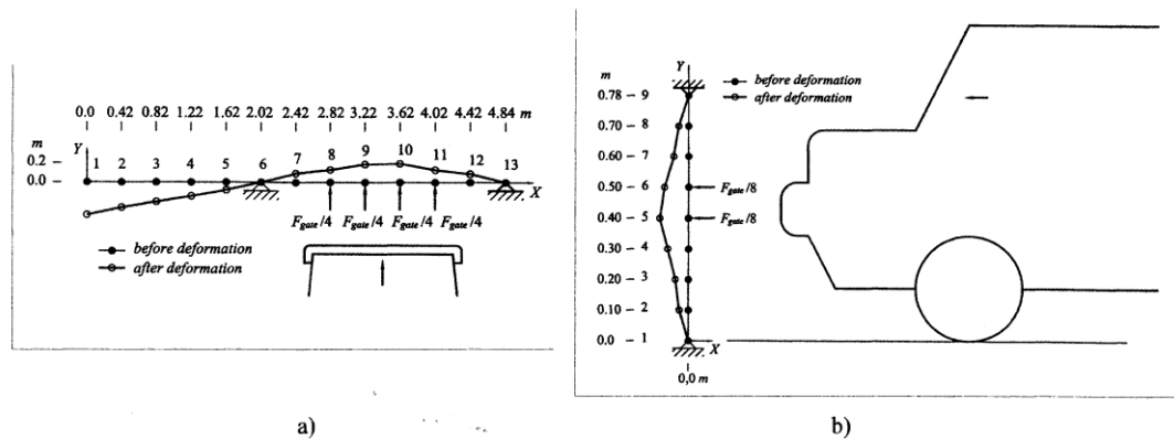
Figure 7. The computational scheme and the outcomes of computer-run simulation
