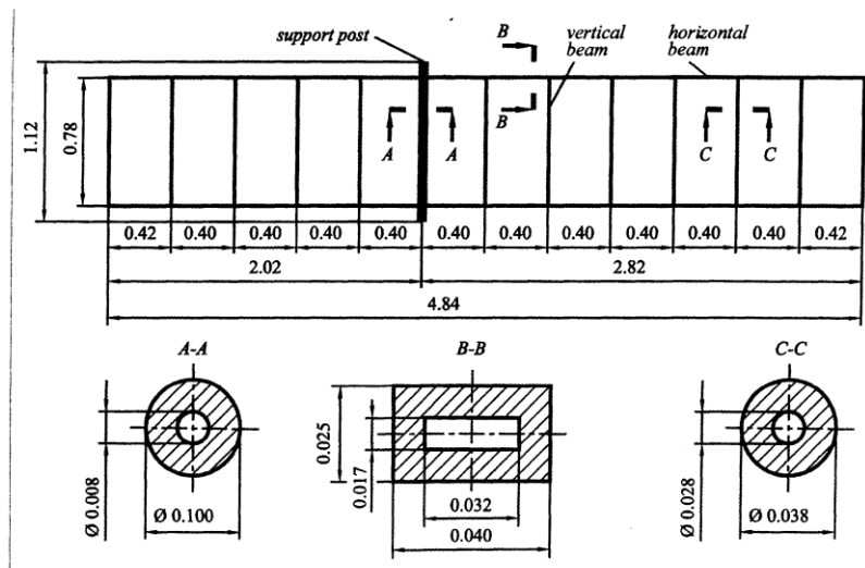
Figure 3. The scheme of the investigated gate
