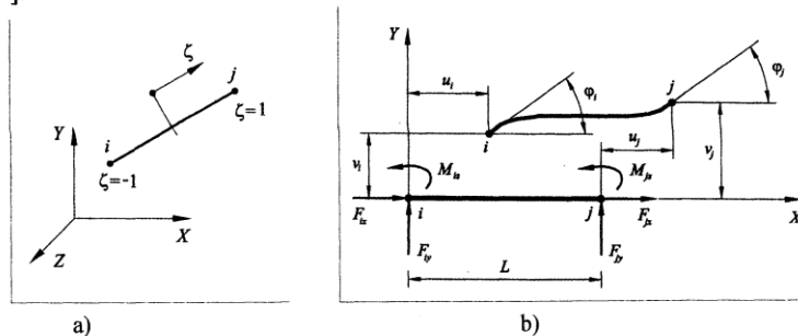
Figure 6. The first-order one-dimensional finite element: a – the scheme within the system of X - Y - Z coordinates; b – the deformations on X - Y plane
