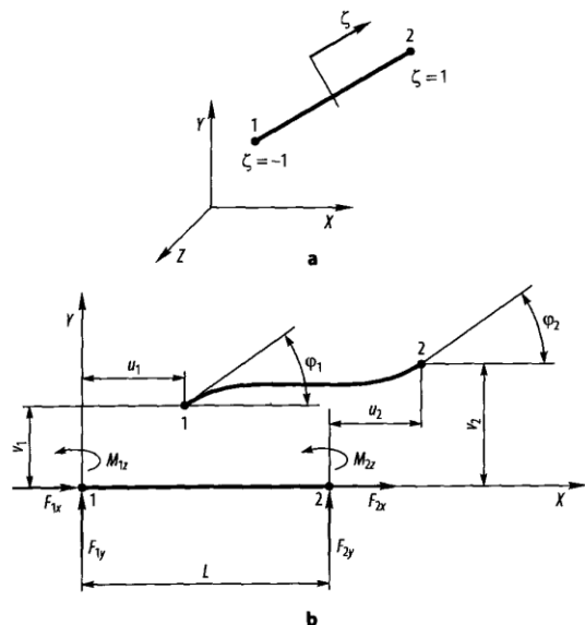
Fig. 6. One-dimensional first-order finite element: a - scheme in the system of the coordinates X - Y - Z; b - deformations in the plane X - Y
