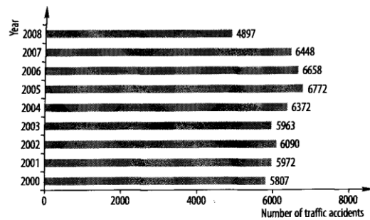
Fig. 1. The dynamics of traffic accidents registered by Highway Patrol Police of Lithuania in 2000–2008
