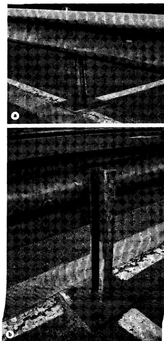
Fig. 5. The elements of metal guardrail: a – protective W-shape horizontal beam (in the foreground); b – \Sigma -shape post (in the foreground)
