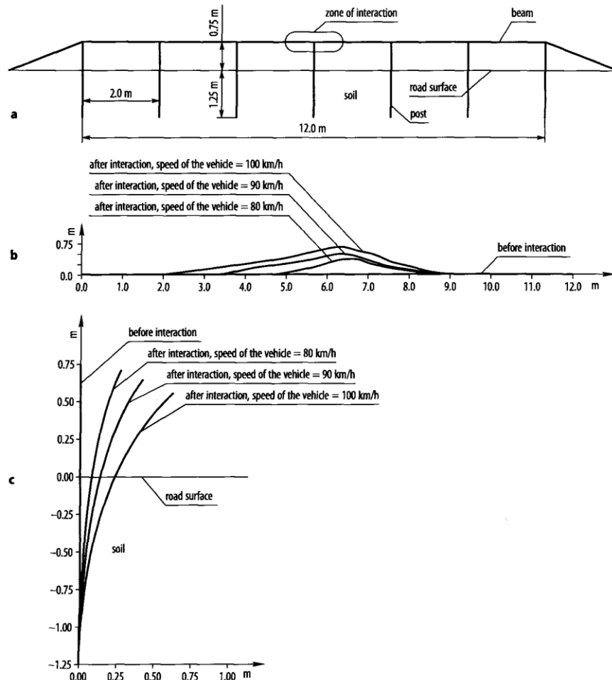
Fig. 7. The deflections of metal road guardrail elements caused by the impact of a vehicle moving at varying speed (angle of interaction between a vehicle and a guardrail – 20°): a – scheme of the metal guardrail; b – deflections of protective W-shape horizontal beam; c – deflections of Σ-shape post
