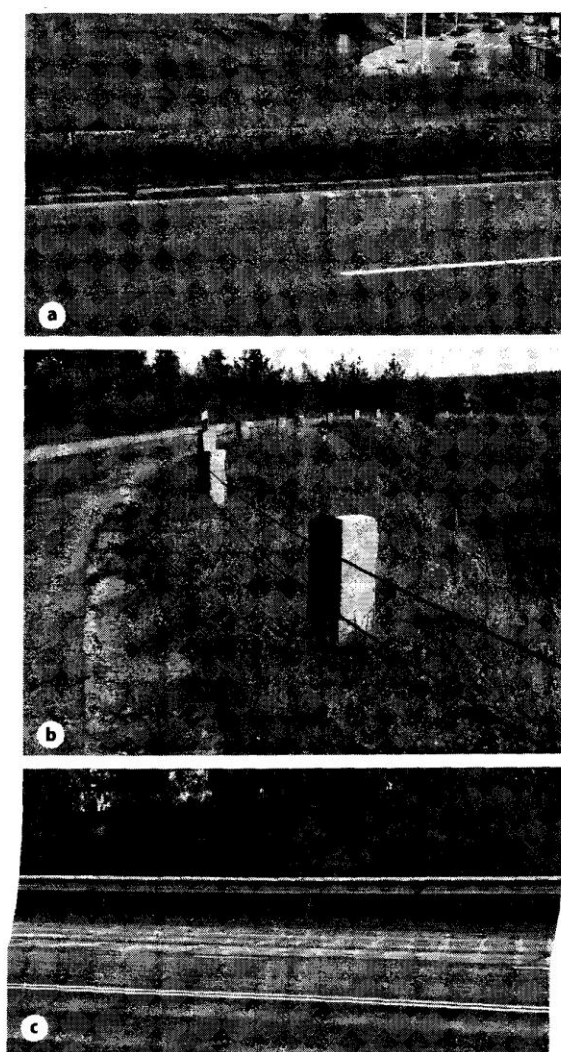
Fig. 4. Guardrails installed on highways: a – reinforced concrete guardrail; b – cable guardrail; c – metal guardrail
