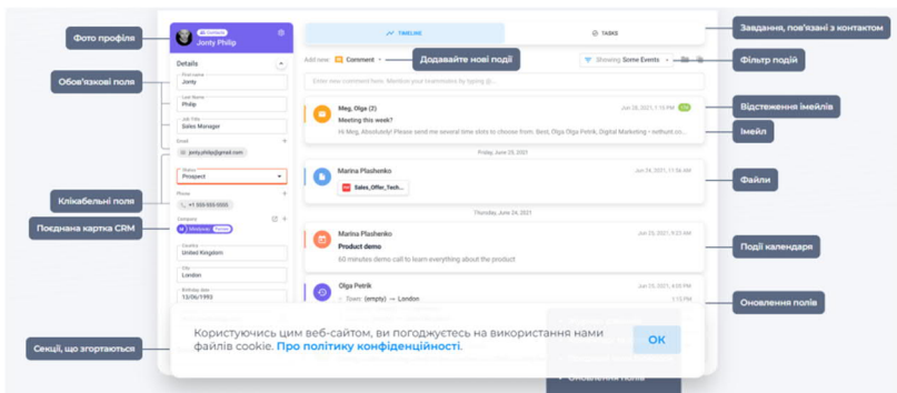
Figure 2 - Interface of NetHunt
