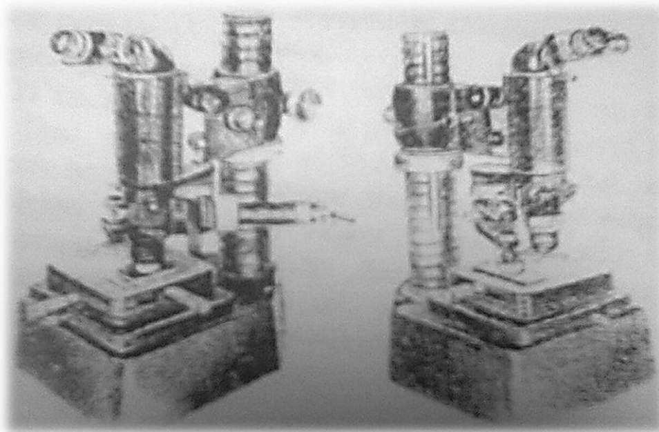
Fig. 3.3. External view of the device PMT - 3
