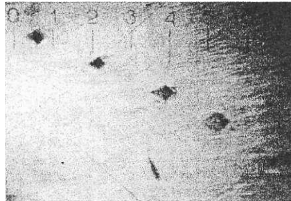
2.2 Dents of the pyramid while determining linear wear.
