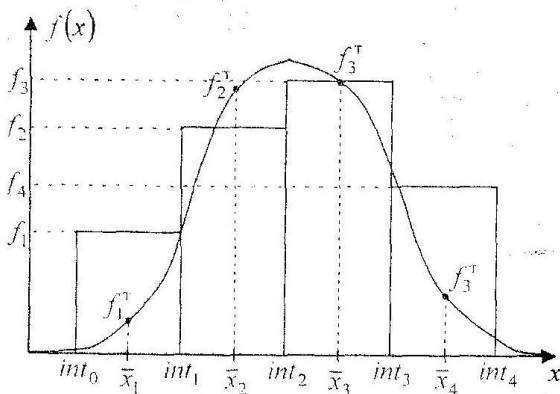
Pic.13 Histogram
