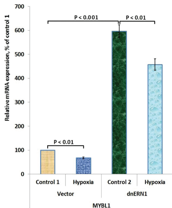
Fig. 1. Effect of hypoxia (3% oxygen – 16h) on the expression level of transcription factor MYBL1 in control U87 glioma cells (Vector) and cells with inhibition of IRE1/ERN1 enzymatic activities (dnERN1) measured by qPCR. The values of MYBL1 mRNA expression were normalized to beta-actin mRNA level and presented as percent of control (100%); n = 4
