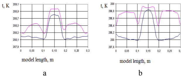
Fig. 2. The temperature distribution along: (a) is the upper boundary layer and (a) is the lower surfaces external contour model for oncoming flow velocity of 40 m/s at a distance from the front edge of the 1/3 chord (blue line) and the 2/3 chord (red line)
