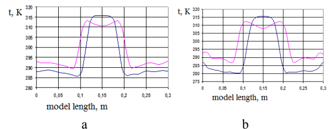
Fig. 4. The temperature distribution along the (a) is the upper boundary layer and (a) is the lower surfaces external contour model for oncoming flow velocity of 240 m/s at a distance from the front edge of the 1/3 chord (blue line) and the 2/3 chord (red line)
