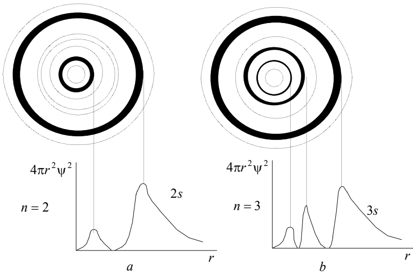
Fig. A2.4. The graphs of the electron cloud of 2s - and 3s -electrons
