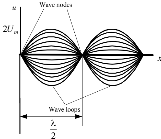
Fig. A1.9. The voltage standing wave (one-dimensional case)
