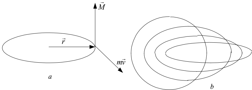
Fig. A2.2. The shapes of the electron cloud
