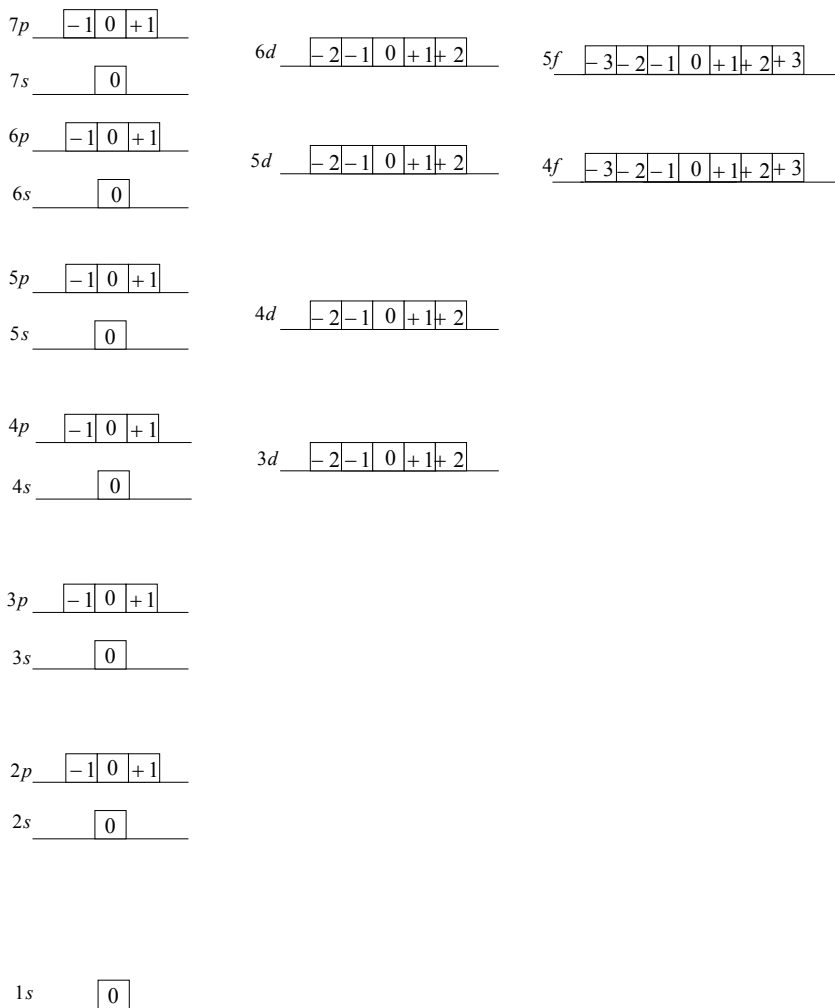
Fig. A2.9. The scheme of mutual arrangement of the energy sublevels in the atom
