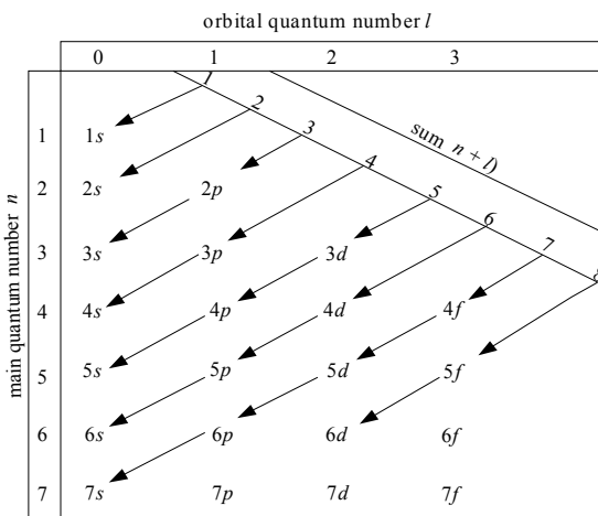
Fig. A1.1. Electron-graphical schemes
