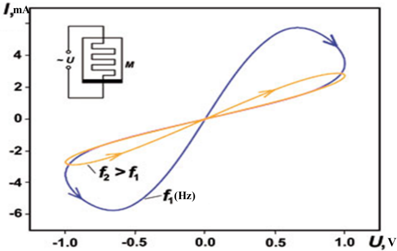
Fig. 1.23. The dependence of the current-voltage characteristics of a memristor from frequency
