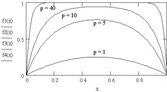
Fig. 2.7. Graphs of the window function f(x) = 1 - \left[ (x - 0,5)^2 + 0,75 \right]^p
