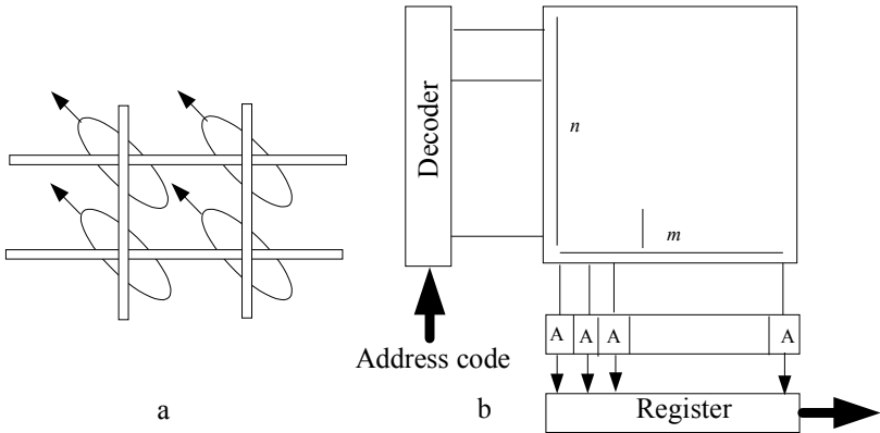
Fig. 7.15. The reading circuit
