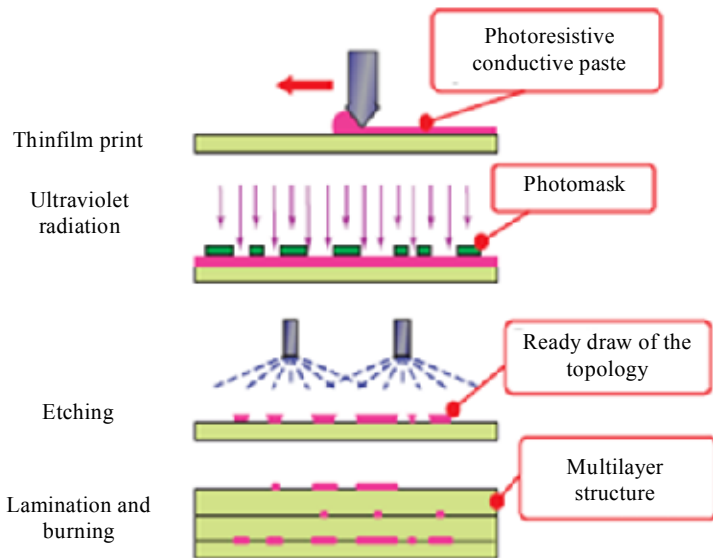
Fig. 6.6. The process of the photolithography
