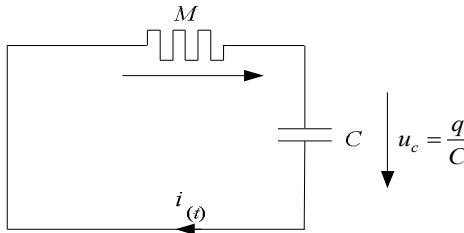
Fig. 4.5. The circuit of discharge of the capacitor
