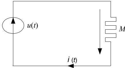
Fig. 4.1. Electrical circuit with the memristor
