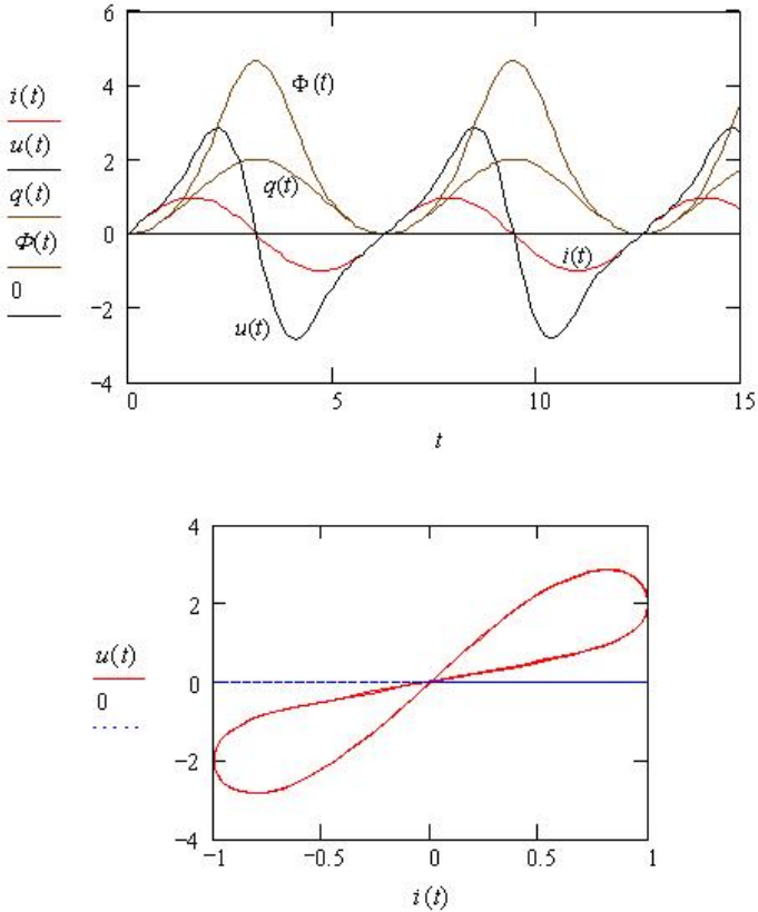
Fig. 1.9. Characteristics of the memristor controlled by charge
