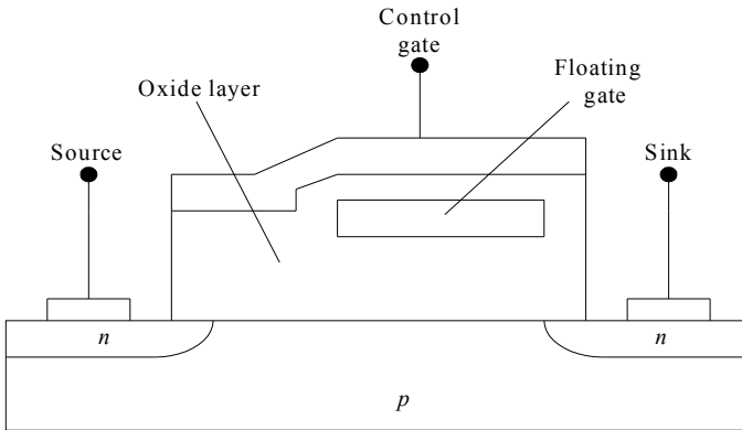
Fig. 7.1. The scheme of the field effect transistor with the floating gate
