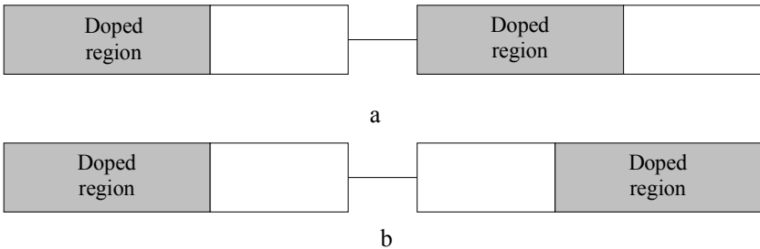
Fig. 4.4. Series connected memristors
