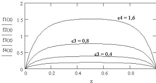
Fig. 2.8. Graphs of the window function f(x) = c \left[ 1 - \left[ (x - 0,5)^2 + 0,75 \right]^p \right]
