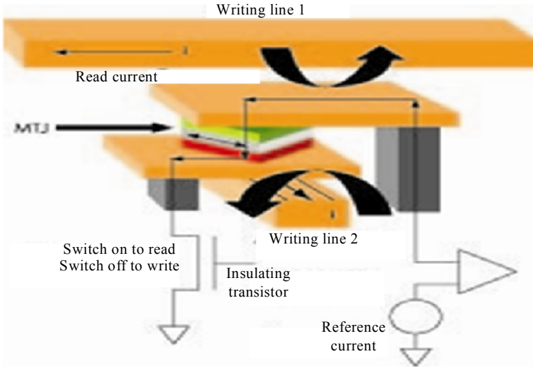
Fig. A3.2. Elementary cell of the MRAM-memory
