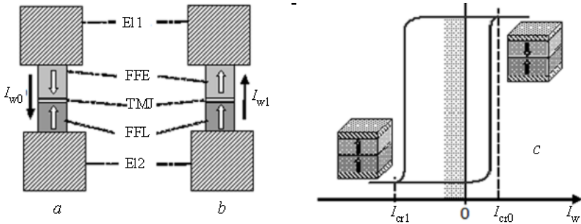
Fig. 7.54. The structural diagram of the memory cell
