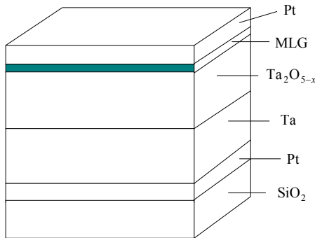
Fig. 7.5. Memory cell structure of the ReRAM type
