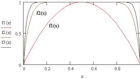
Fig. 2.3. Graphs of window function for different values of parameter p
