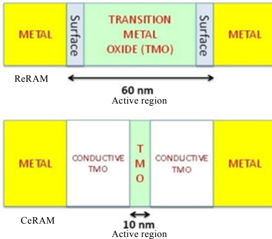
Fig. 7.38. Structures of the ReRAM and CeRAM
