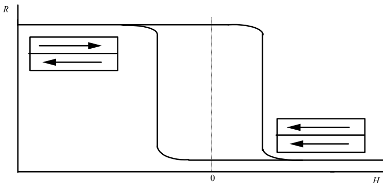
Fig. 7.14. The switching of the states in the MRAM cell
