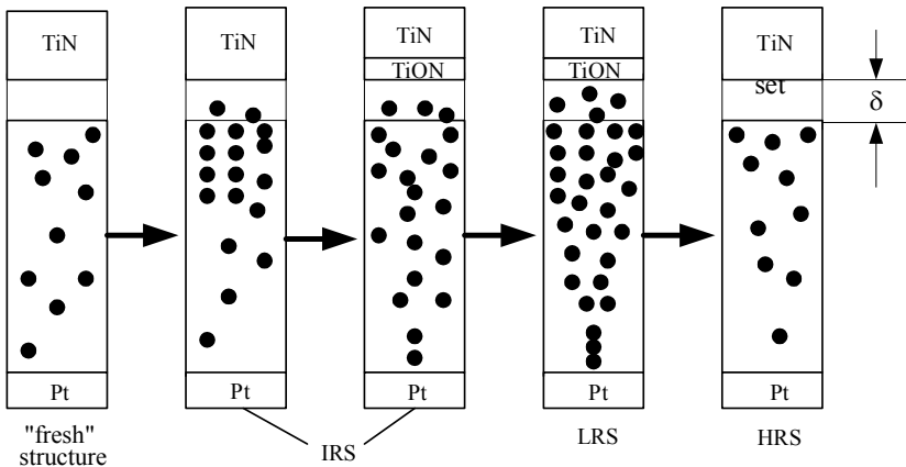
Fig. 5.14. Formation of the intermediate states of the structure
