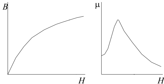
Fig. A1.3. The dependencies of the magnetic induction B and the magnetic permeability \mu from the magnetic field intensity H
