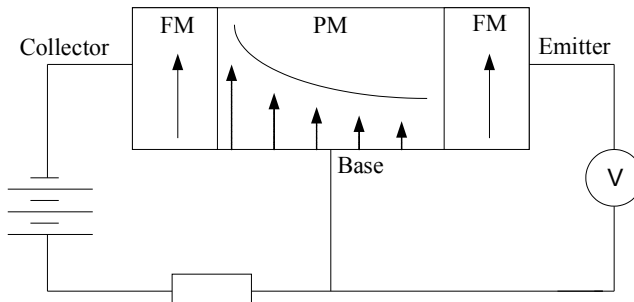
Fig. 7.11. The structure of the Jonson transistor
