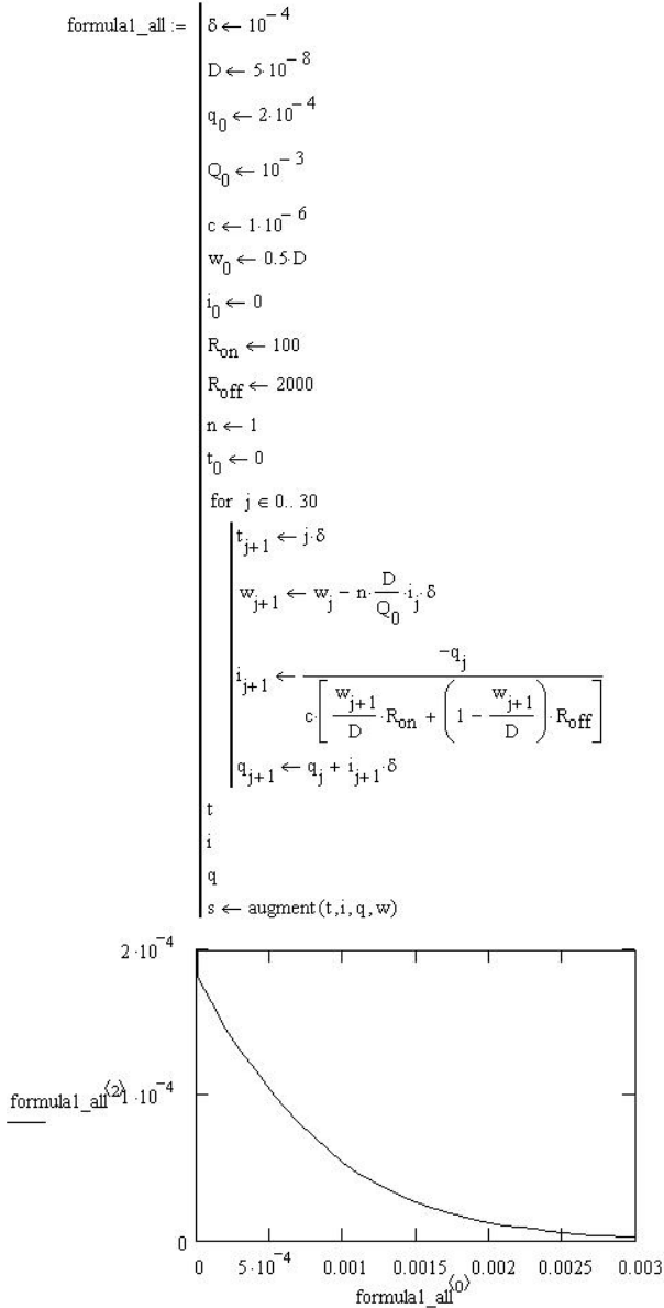
Fig. 4.6. The numerical integration of the nonlinear differential equation gives q-t graph
