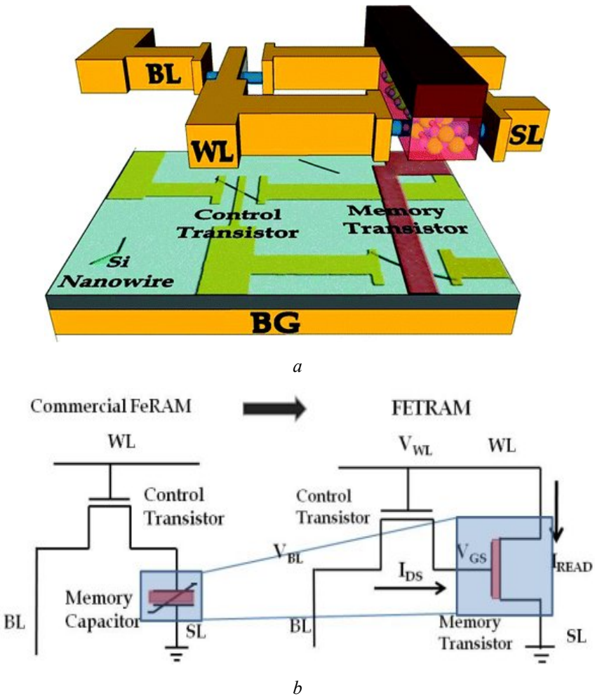
Fig. 7.34. (a) is the structure of the FeTRAM cell; (b) is the scheme of the cell
