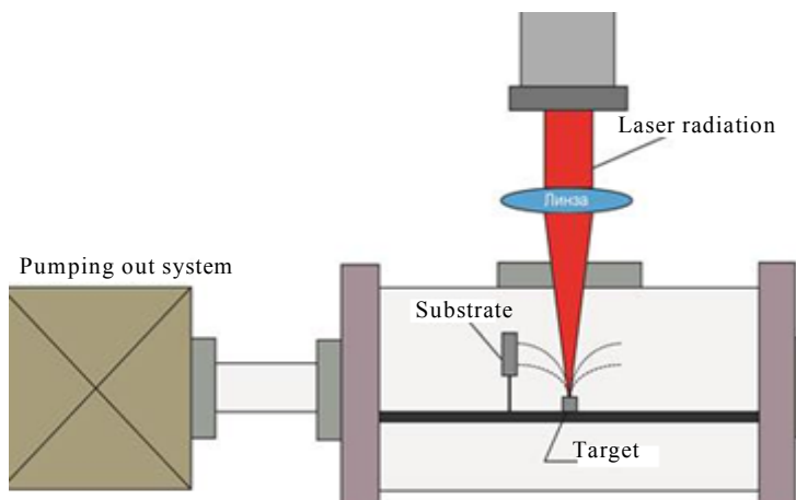
Fig. 6.17. Laser ablation of the target material
