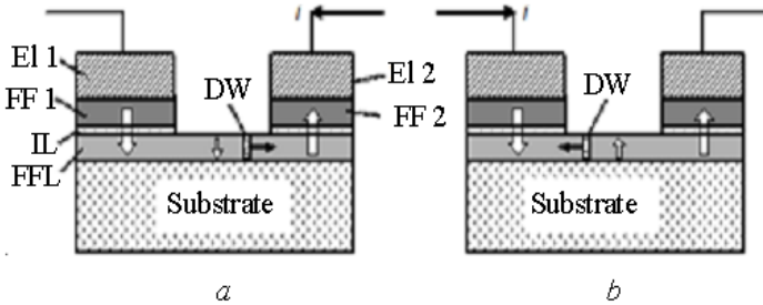
Fig. 7.43. Process of the spin-transport magnetization reversal
