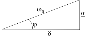
Fig. 4.11. The relationships between the frequencies in RLC -circuit Finally we have:
