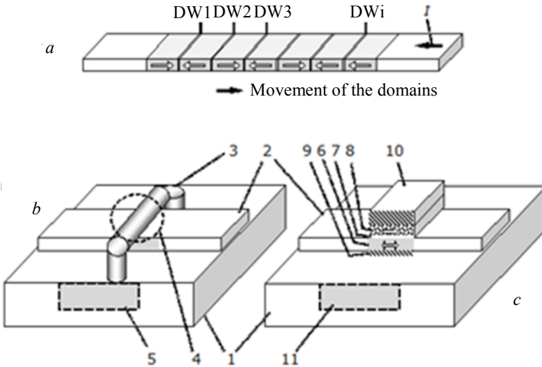
Fig. 7.47. Movement of the domains (a), writing (b) and reading units (c)
