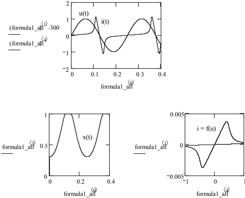
Fig. 2.9. Characteristics of the nonlinear model of the memristor with the window function f(x) = x - x^2
