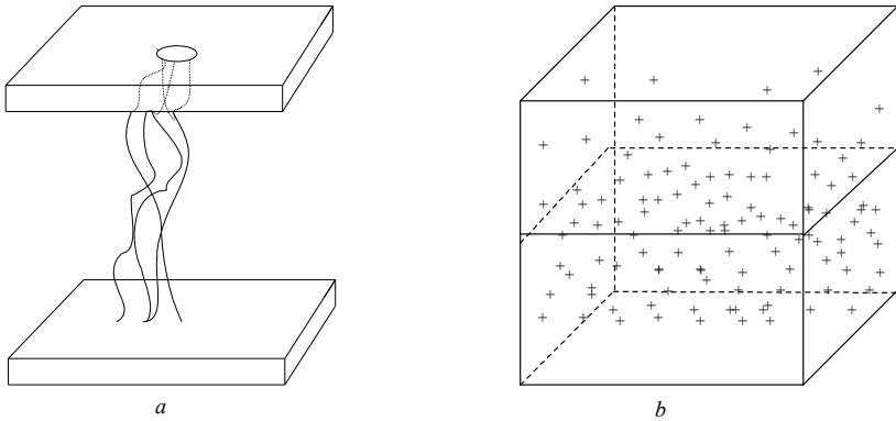
Fig. 5.11. The methods of the resistive switching: a : filamentary switching process in which the conductivity of the active region is limited by the thread (threads) and the switching occurs within that thread; b : uniform switching process (VCM), for which the entire active region located under the metal electrode, participates in the process of switching
