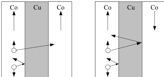
Fig. 7.9. Examples of the magnetic moments of the adjacent ferromagnetic layers
