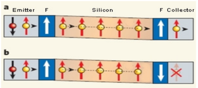
Fig. A3.5. The functioning of the injector and detector: (a) shows layers of CoFe and NiFe which are magnetized in parallel; (b) shows layers which are magnetized in antiparallel, F is the first and second ferromagnetic layers
