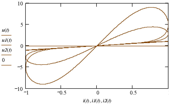
Fig. 1.12. Change CVC of the memristor with increasing frequency of the acting signal
