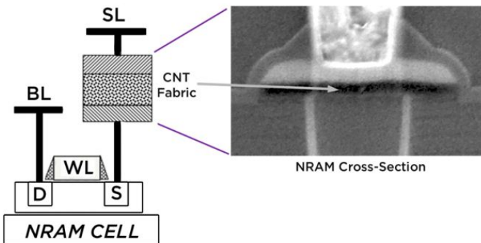
Fig. 7.53. The structure of the NRAM cell and the image of its cross-section
