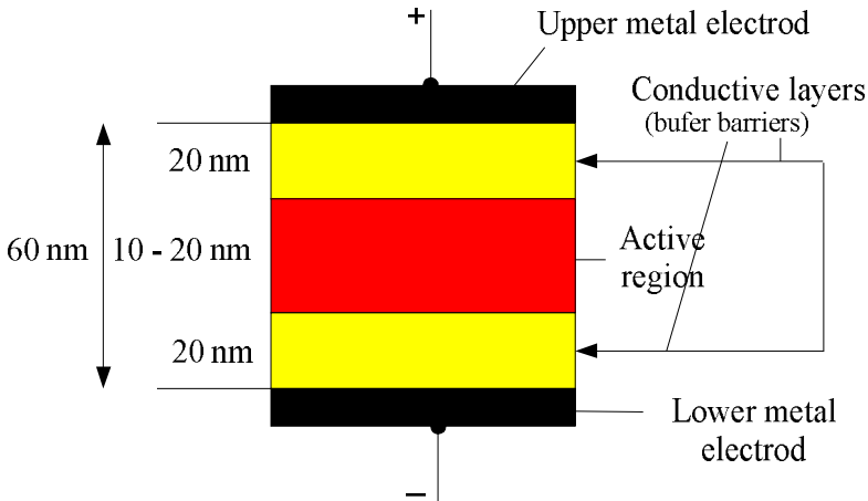
Fig. 7.37 The structure of the CeRAM memory cell
