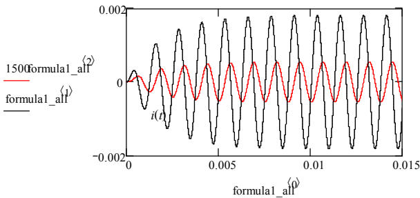
Fig. 4.16. Transient process in the MLC -circuit for \omega \approx \omega_0
