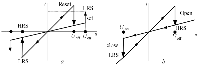
Fig. 5.8. Unipolar (a) and bipolar (b) the memristor switching
