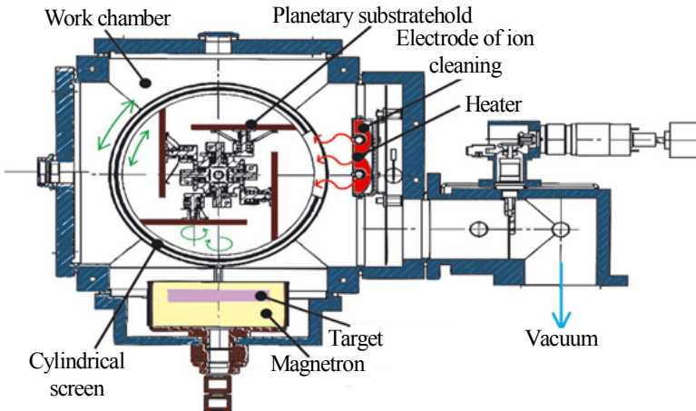
Fig. 6.13. Block diagram of the magnetron deposition plant
