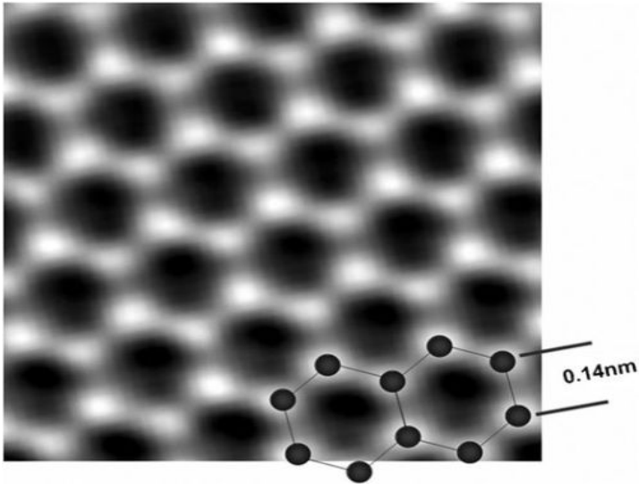
Fig. 7.6. Image of the graphene structure obtained by the atomic force microscope
