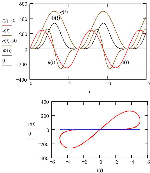
Fig. 1.11. The response of the memristor on the amplitude of action equaled I_m = 5 A
