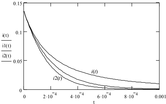
Fig. 4.9. The graphs of the transients in the ML -circuit
