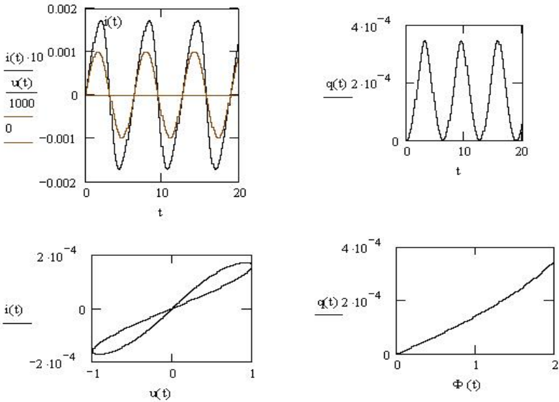
Fig. 2.1. Graphs of dependencies u(t) , i(t) , q(t) , \Phi(t) , i = f(u) for the linear model of the memristor
