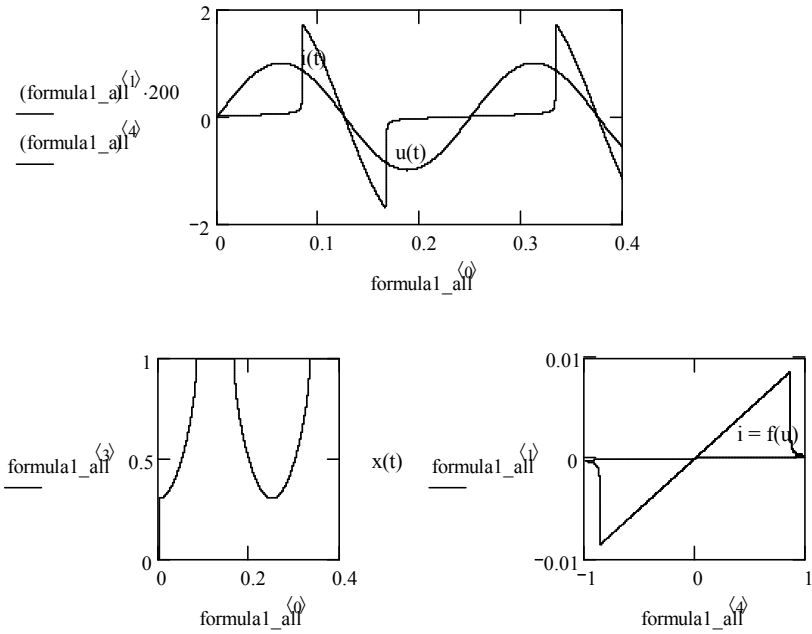
Fig. 2.10. Characteristics of the nonlinear model of the memristor with the window function f(x) = 1 - (2x - 1)^{2p} with the parameter p = 9
