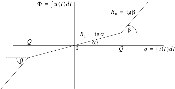
Fig. 5.1. The veber-coulomb characteristic of the memristor
