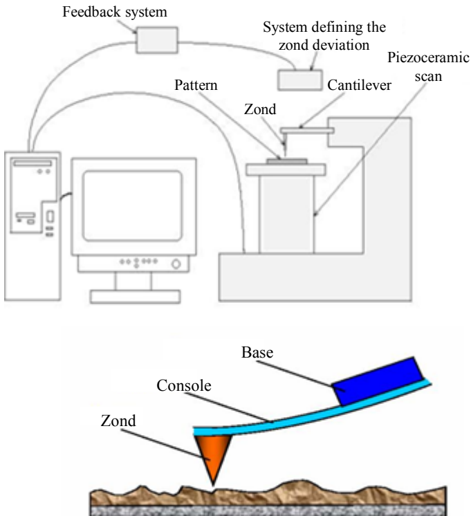
Fig. 6.2. Principle of operation of the atomic force microscope
