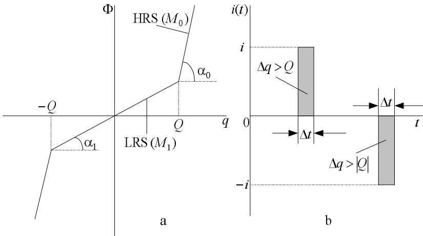
Fig. 5.17. The signals of the bipolar switching of the memristor
