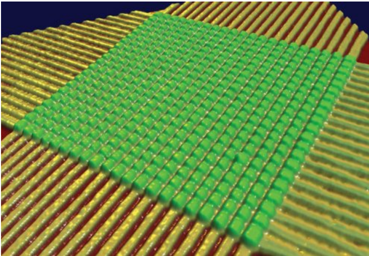
Fig. 6.1. The image of the matrix of the memristors in the atomic force microscope
