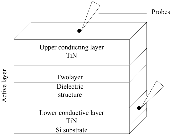
Fig. 6.18. Position of the probes with respect to the sample
