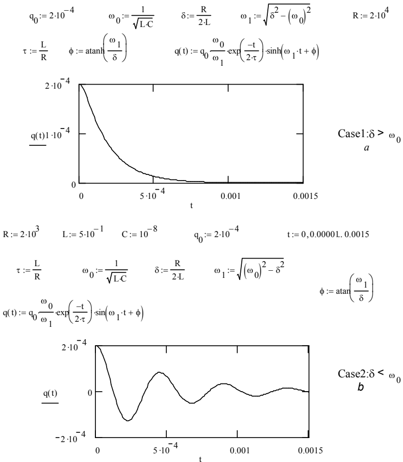
Fig. 4.12. The transients of the capacitor discharge
