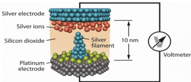
Fig. 5.13. Formation of the filament in the structure Ag/SiO 2 /Pt
