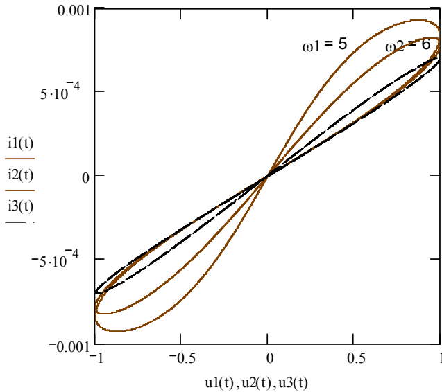
Fig. 4.3. Volt-ampere characteristics of the memristor
