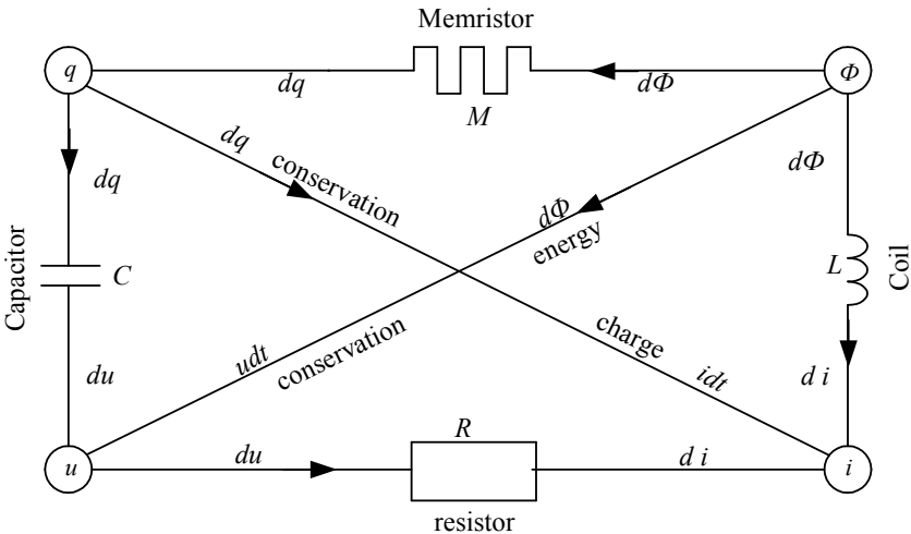
Fig. 1.2. Interconnection between the fundamental variables of electric circuits
