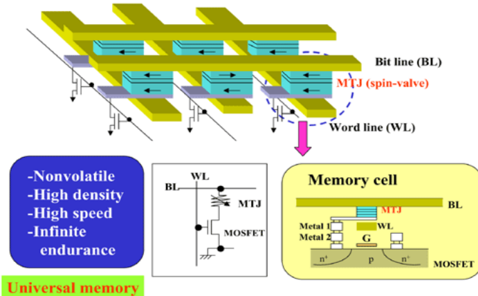
Fig. 7.17. The technology of manufacturing the memory matrix
