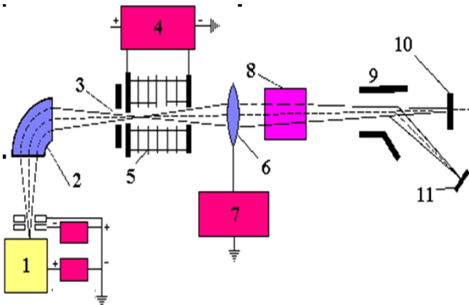
Fig. 6.10. A block diagram of an ion implantation
