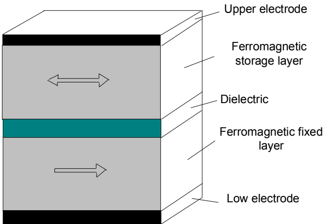
Fig. 7.13. The structure of the elementary cell
