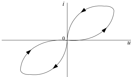
Fig.1.1. Current-voltage characteristic of a memristor
