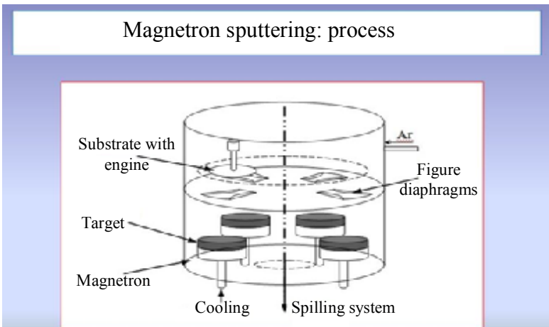
Fig. 6.12. Magnetron sputtering process
