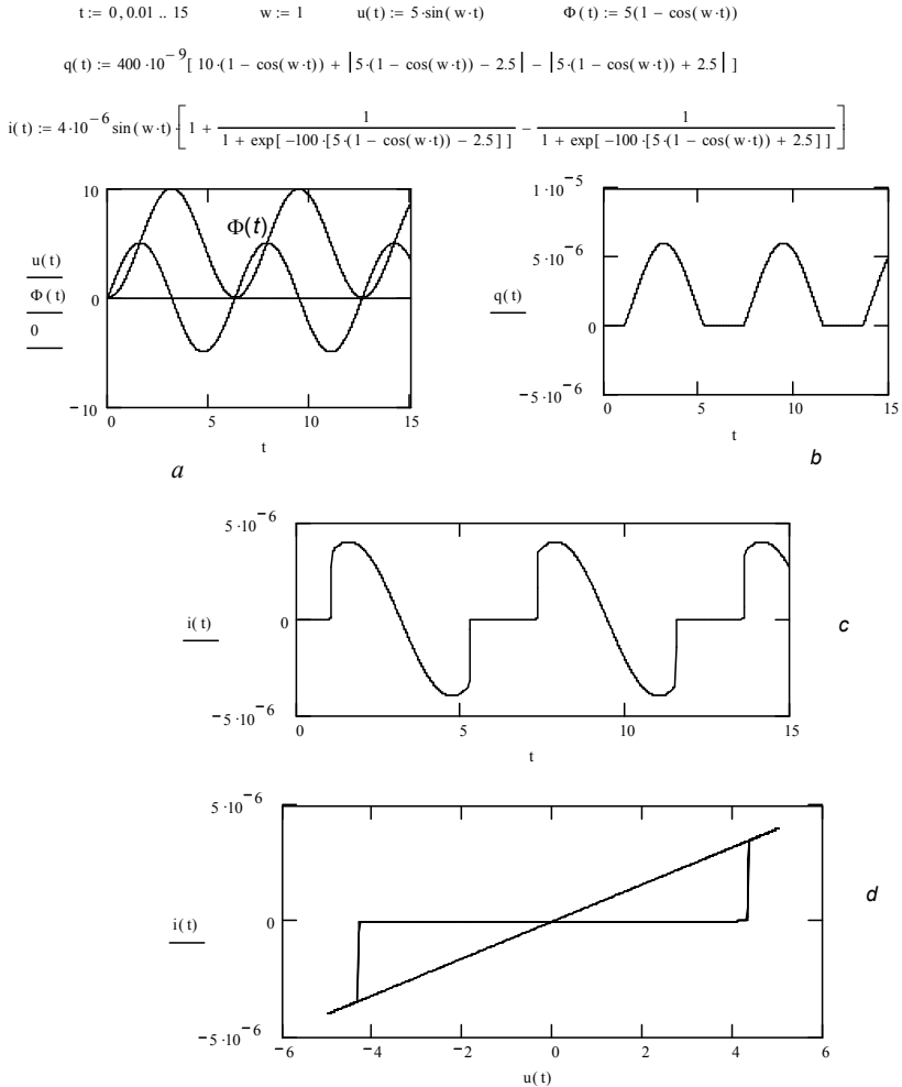
Fig. 5.6. Basic dependencies of the resistive switching
