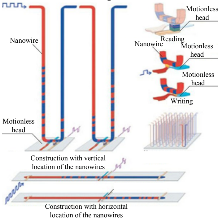
Fig. 7.44. The ways of the nanowire location
