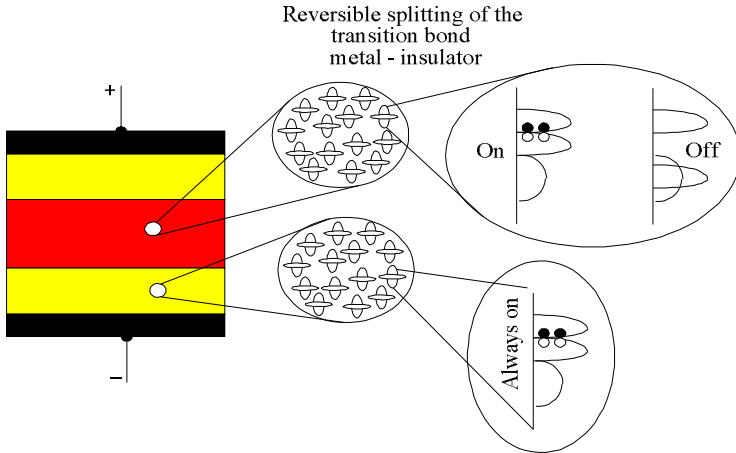
Fig. 7.39. The local zone structures for different states of the conductance
