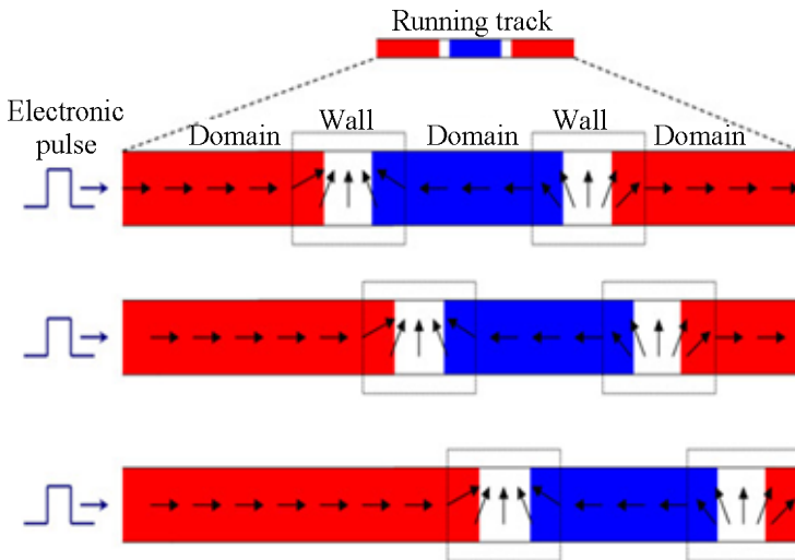
Fig. 7.42. Movement of the domain walls under the acting of the spin-polarized electric current
