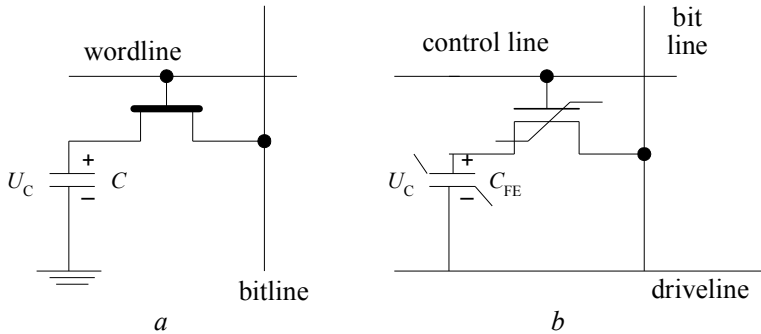
Fig. 7.32. Memory cell DRAM type (a) and 1T-1C FeRAM type (b)
