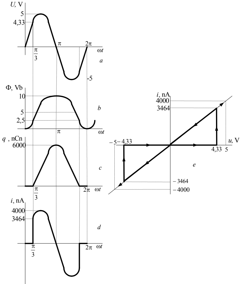
Fig. 5.5. Theoretical graphs of the basic dependencies
