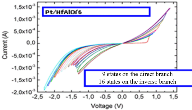
Fig. 5.15. The experimental current-voltage characteristics of the memristor with several intermediate states
