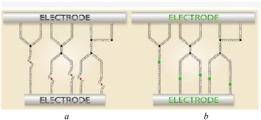
Fig. 7.52. The functioning diagram of the NRAM memory cell for the disconnection of the nanotubes (a) and their connection (b)
