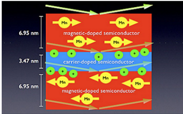
The thin magnetic layers of the semiconductor (red) separated by the nonmagnetic layer (blue) may demonstrate the phenomenon known as the antiferromagnetic relation when the atom of the manganese (Mn) is magnetized in the opposite direction on the adjacent magnetic layer
