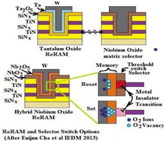
Fig. 7.4. Multilayer structures of the ReRAM memory cells
