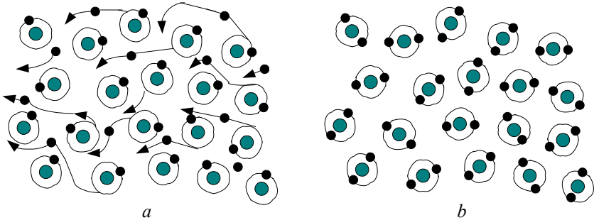
Fig. 7.41. The schematic difference between the states metal-insulator at the level of the nickel ions
