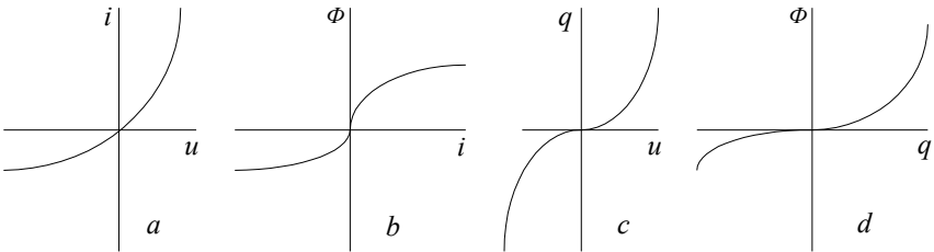
Fig. 1.15. Characteristics of the four fundamental elements
