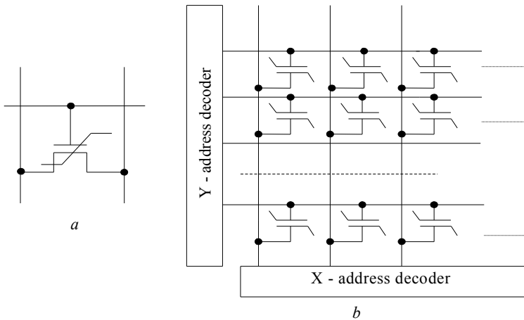
Fig. 7.31. (a) is the scheme of the 1TFeRAM cell type; (b) is the memory type 1SFeRAM (each cell contains one ferroelectric capacitor)
