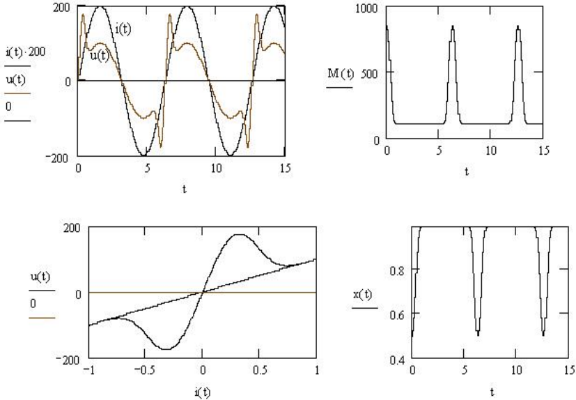
Fig. 2.4. Simulation results of the memristor described by the Nonlinear model
