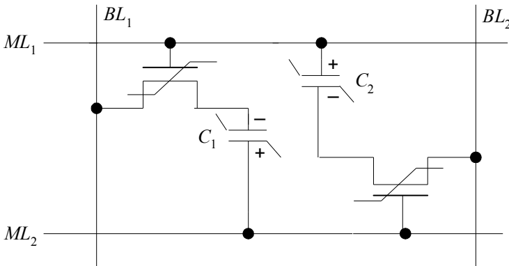
Fig. 7.33. Memory cell 2T-2C FeRAM type
