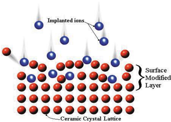
Fig. 6.9. The ion implantation process
