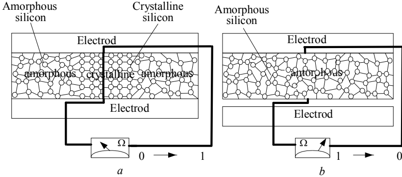
Fig. 7.27. Crystalline and amorphous states of the PCRAM memory cell
