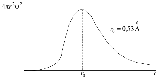
Fig. A2.3 The graph of the probability distribution of finding electron in the hydrogen atom
