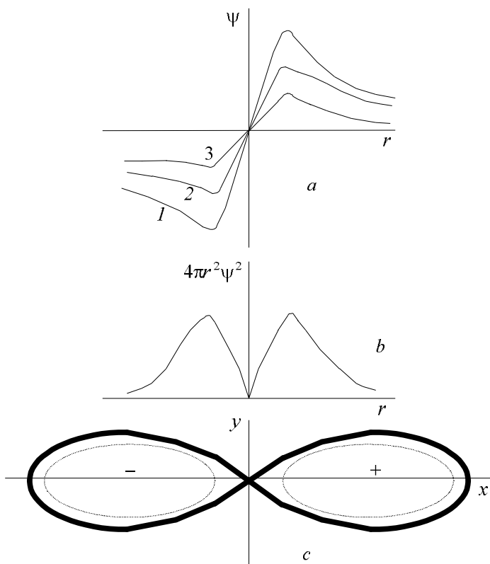
Fig. A2.5. The graphs of the functions \psi and \psi^2 for 2p -electrons
