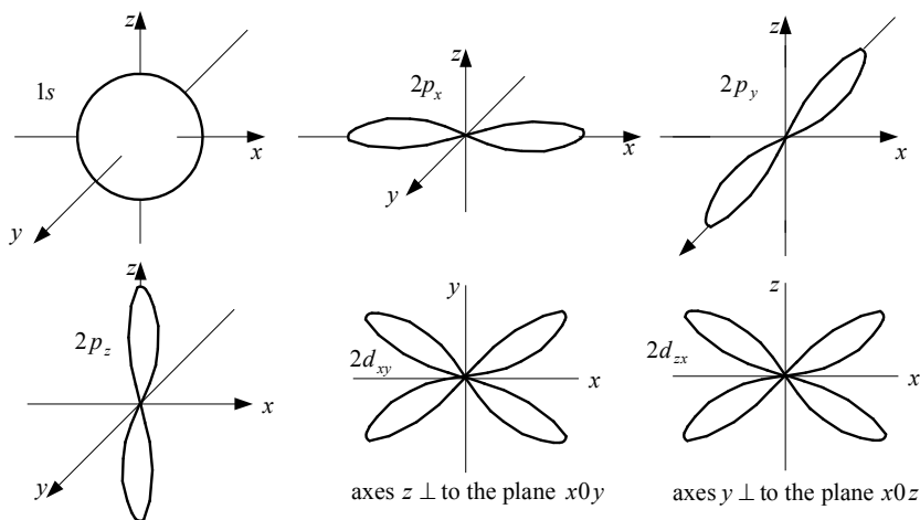
Fig. A2.8. Location of the electron clouds in the space
