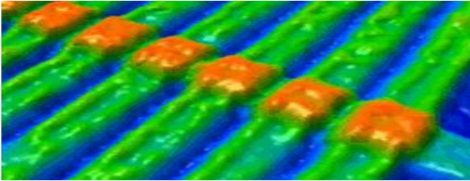
Fig. 5.10. The image of the memristors in the nodes of the matrix structure
