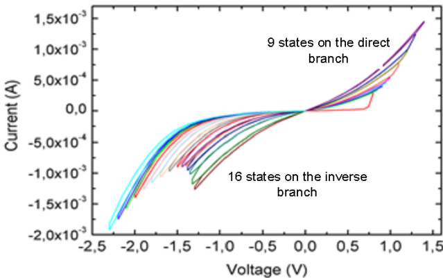
Fig. 6.20. Current-voltage characteristics of the intermediate states of the memristor
