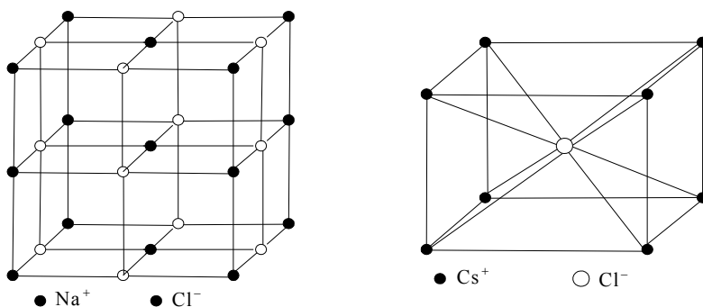
Fig. 7.26. The elementary cells of the lattices
