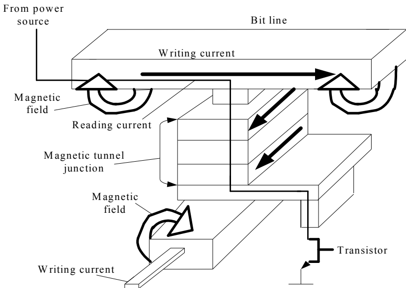
Fig. 7.18. Elementary cell of the MRAM memory
