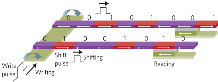
Fig. 7.46. Writing and reading operations used in the horizontal location of the nanowires
