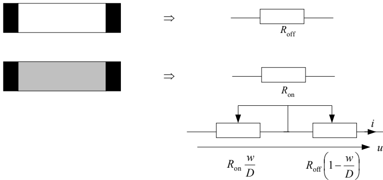
Fig. 1.21. The change of the memristor resistance according to its state
