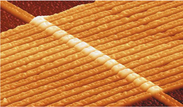
Fig. 1.18. Crossbar including 17 memristors
