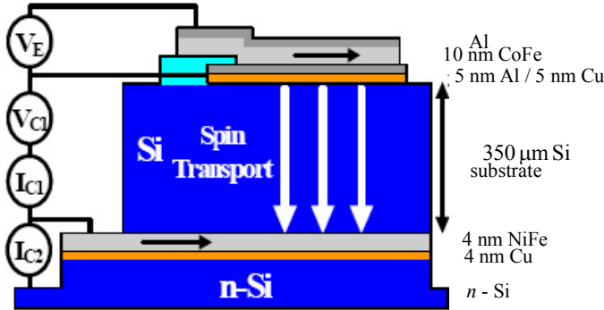
Fig. A3.4. The scheme of the spin transistor functioning
