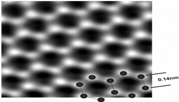
Fig. 7.23. Resolution of the scanning tunneling microscope
