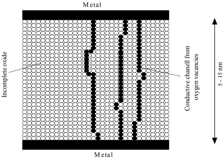
Fig. 5.12. Formation of the filaments in the resistive switching process
