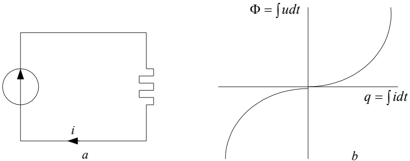
Fig. 1.8. Weber-Coulomb characteristic of the memristor
