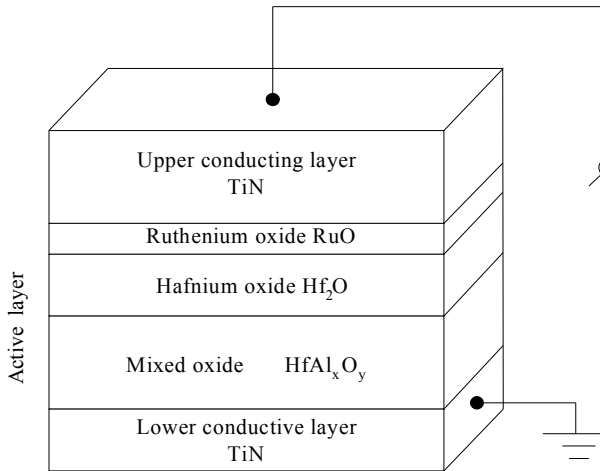
Fig. 6.11. The general structure of the memristor
