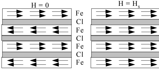
Fig. A3.1. Antiferromagnetic exchange coupling
