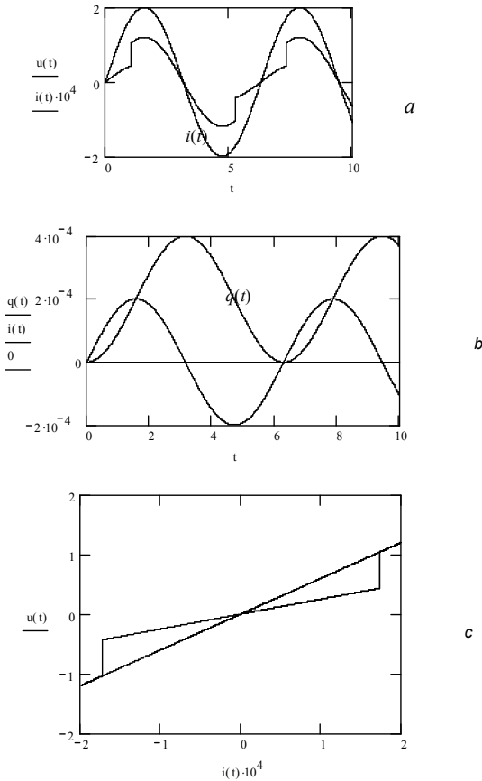
Fig. 5.3. Basic dependencies of the memristor controlled by the charge
