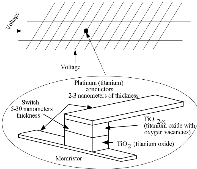
Fig. 1.6. Monolayer matrix of memristors
