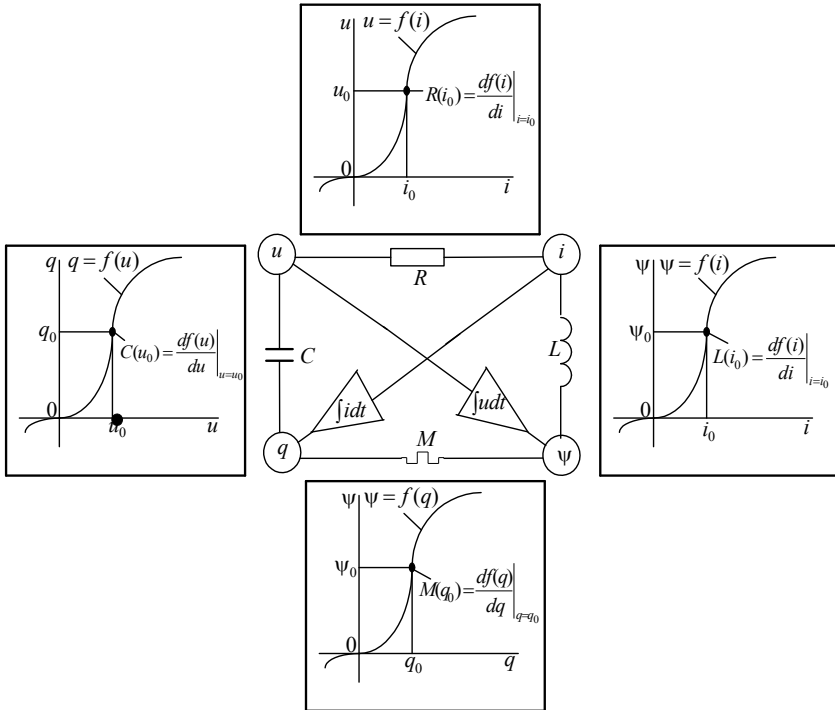
Fig. 1.7. Slope characteristics of fundamental elements
