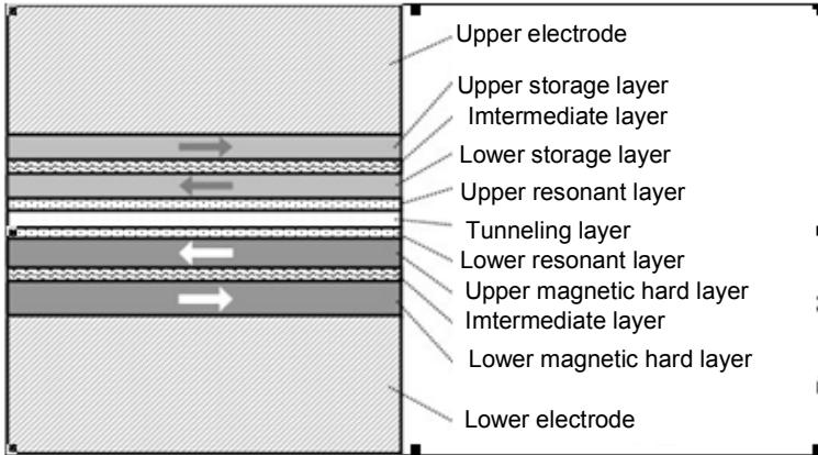
Fig. 7.20. Multilayer architecture of the MRAM cell
