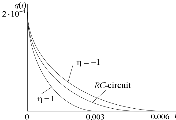
Fig. 4.7. Graphs q(t) for different values of \eta
