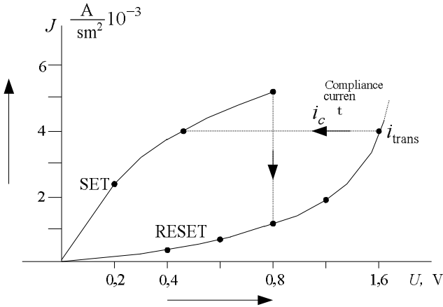
Fig. 7.36. Current-voltage characteristic of the CeRAM cell
