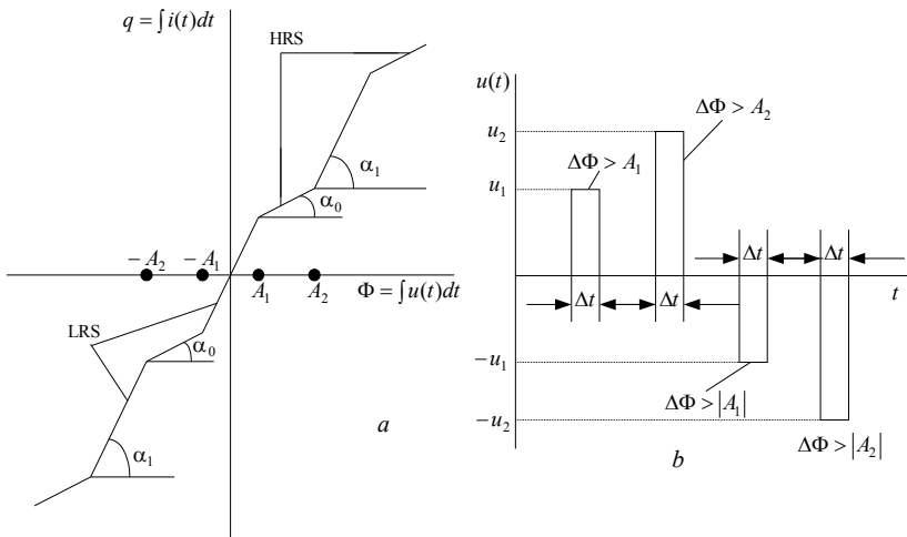
Fig.5.18. The signals of the unipolar switching of the memristor
