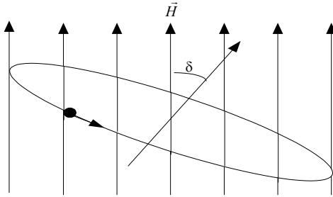
Fig. A2.6. The orientation of the orbit of the electron
