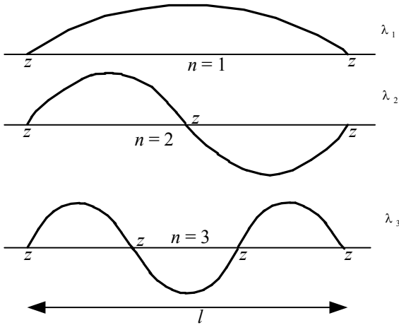
Fig. A2.1. The de Broglie waves for different values n
