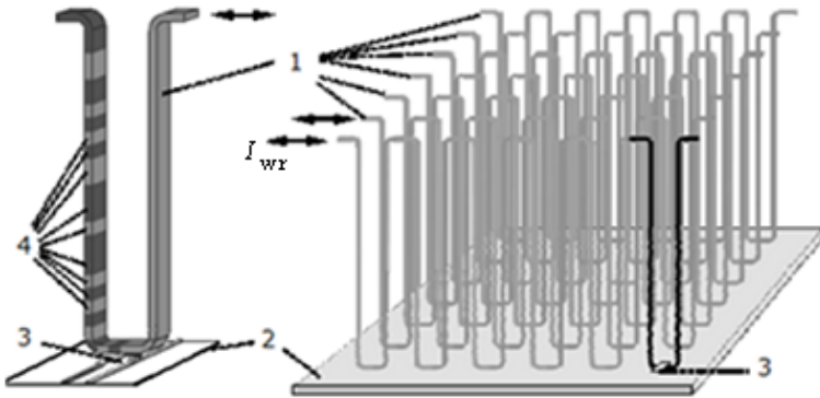
Fig. 7.48. The organization of the three-dimensional memory
