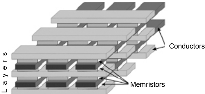
Fig.7.2. Forming 3D structure of the ReRAM memory
