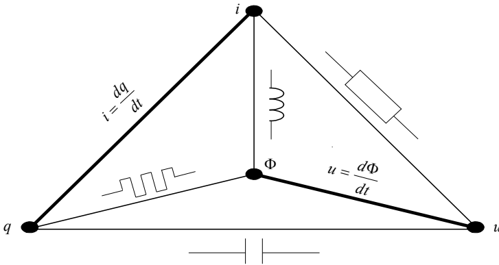
Fig. 1.3. Interconnection between the current, voltage, charge and magnetic flux
