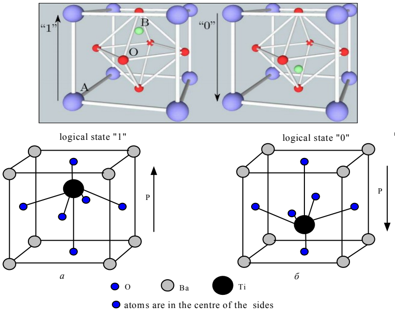
Fig. 7.28. The elementary cell of the barium titanate
