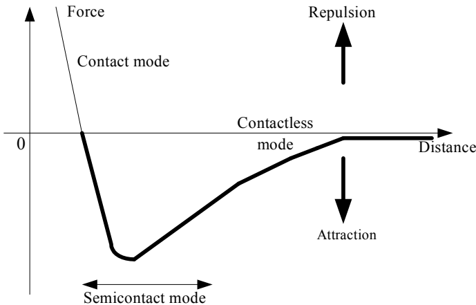
Fig. 6.3. The graph of the dependency of the Van der Waals force from the distance between the console and the sample surface
