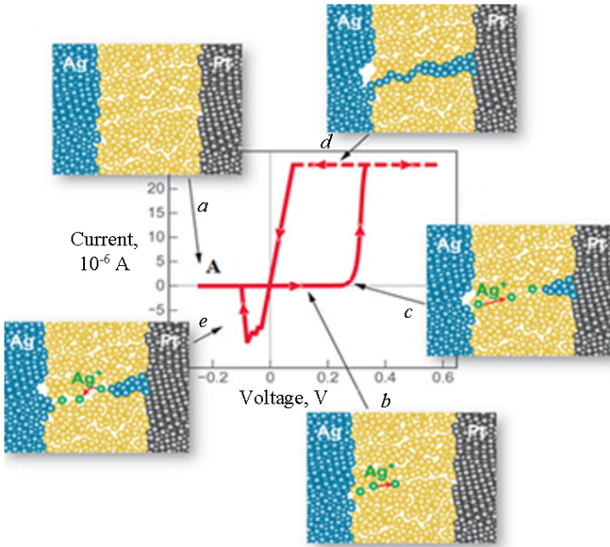
Fig.5.16. The stages of the formation and destruction of the filaments
