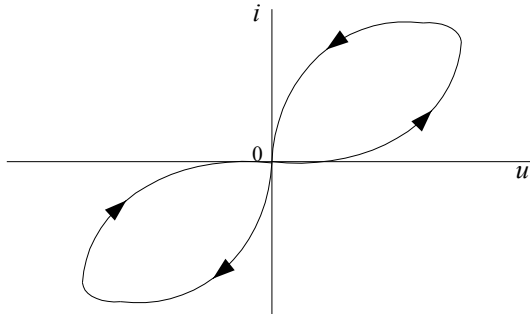
Fig. 1.22. The dependency i(u) of the memristor
