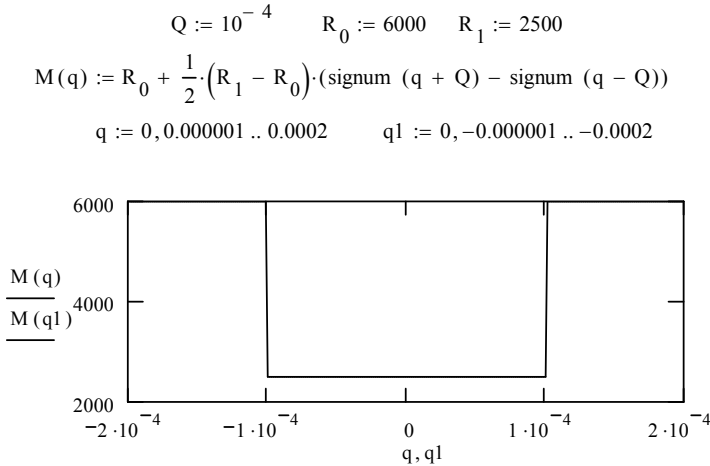
Fig. 5.2. The dependency of the memristance from the charge
