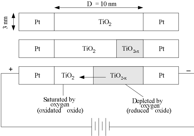
Fig. 5.9. Process of the oxidation | reduction in the MDM structure
