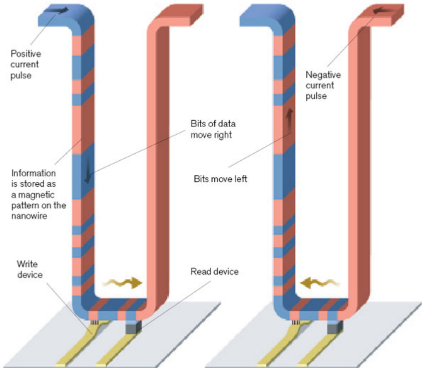
Fig. 7.45. Writing and reading operations used in the vertical location of the nanowires
