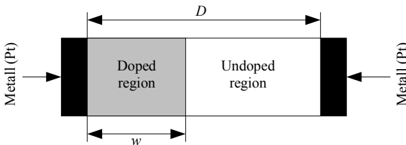
Fig. 1.19. A simple physical model of the memristor
