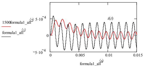
Fig. 4.15. Transient process in the MLC -circuit for \omega > \omega_0
