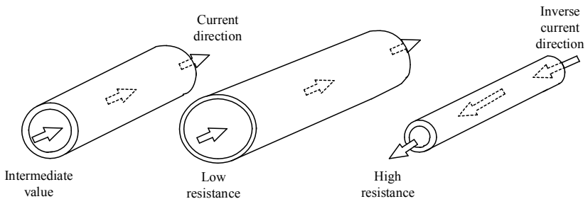
Fig. 1.17. Physical analogy of the memristor
