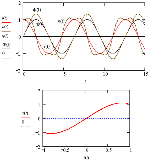
Fig. 1.13. Hysteresis loop degenerates into single-valued function
