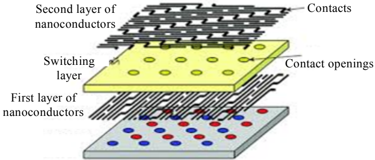
Fig. 1.5. Realization of multi-layer matrixes
