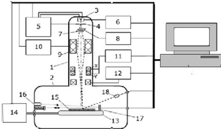
Fig. 6. 5. Block diagram of the electronic lithography system
