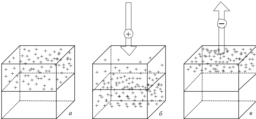
Fig. 1.20. The distribution of oxygen vacancies, depending the polarity of the applied voltage
