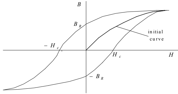
Fig. A1.4. The normal magnetization curve of the ferromagnetic
