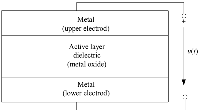
Fig. 5.7. MDM structure of the memristor
