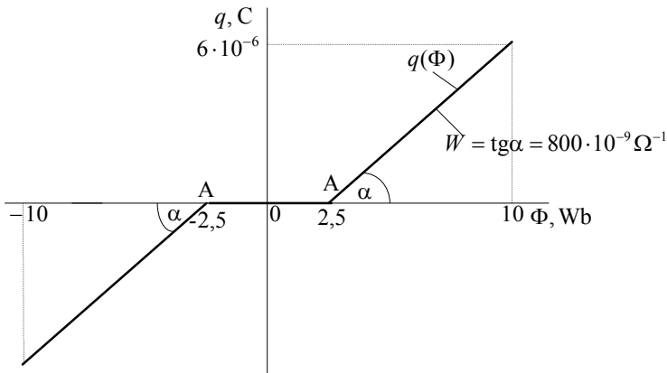
Fig. 5.4. Coulomb-weber characteristic of the memristor
