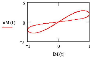
Fig. 1.16. Current-voltage characteristics of the fundamental elements
