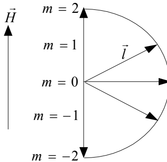
Fig. A2.7. The vector representation of the orbital quantum number
