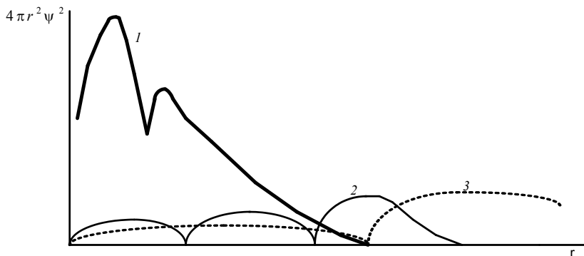
Fig. 7.40. The probability distribution of the electron "clouds"
