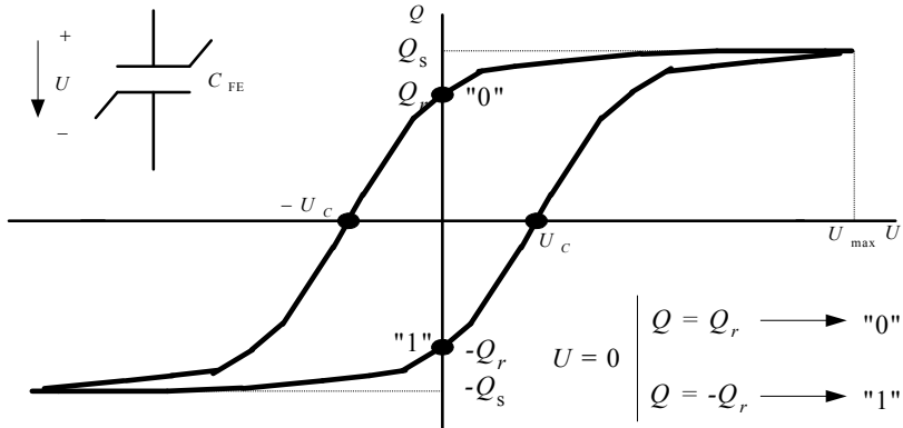
Fig. 7.30. The hysteresis loop of the ferroelectric capacitor
