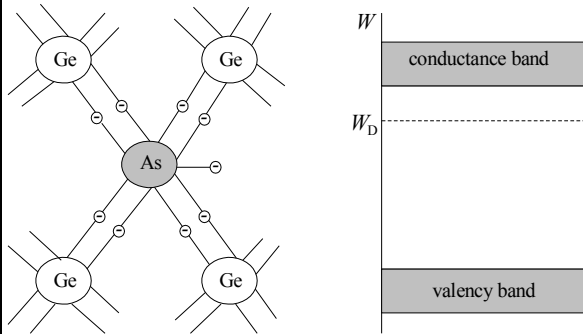
Fig. A1.6. Donor impurity provides the electron conductance of the semiconductor
