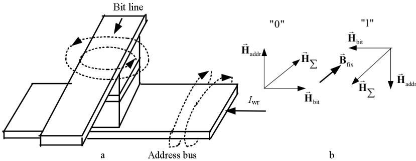
Fig. 7.16. The writing of the information into the chosen cell
