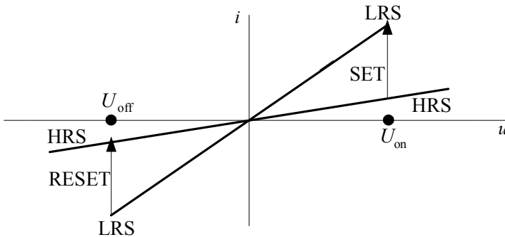
Fig. 6.19. Measurement of the CVC of the RESET and SET processes
