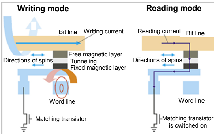
Fig. 7.19. Principle of writing and reading information
