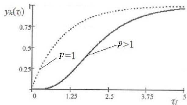
Fig. 2. The logistic function: p_j > 1 is exponent, which emphasizes logistical nature of learning (hastobeidentified); y_k is band which characterizes the quality of education; \tau_j is time dedicated for education
