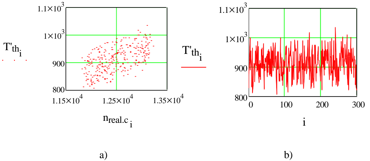
Figure 4.3 Normal measured values of temperature before working turbine along different operation regime with accounting measuring errors.
