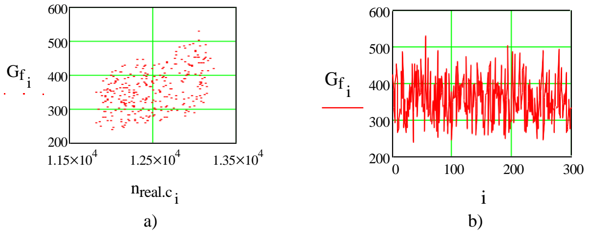
Figure 4.4 Normal measured values of mass fuel consumption along different operating regime with accounting measuring errors.
