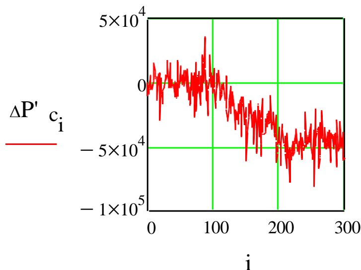
Figure 4.9 Pressure after compressor measured parameter deviation.
