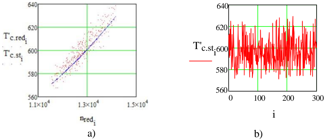
Figure 4.6 Comparison of normal measured temperature after compressor and ideal measured parameter ( T'_{c,red} – normal, T'_{c,st} – ideal).
