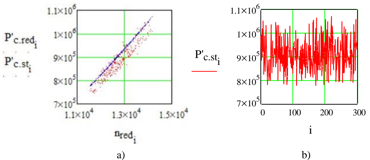
Figure 4.5 Comparison of normal measured pressure after compressor and ideal measured parameter ( P'_{c.red} – normal, P'_{c.st} - ideal).
