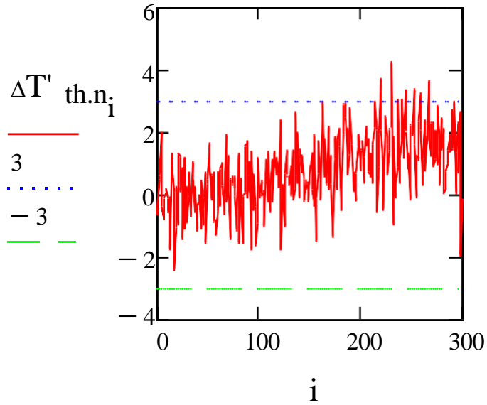
Figure 4.15 Normalized turbine temperature diagnostic deviation dependence from the measurement number.
