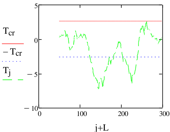
Figure 4.17 Statistic dependence of the Student's distribution with critical boundaries for pressure after compressor parameter.
