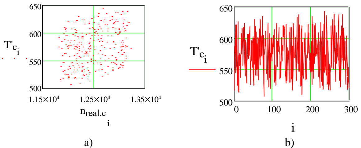
Figure 4.2 Normal measured values of temperature after compressor along different operation regime with accounting measuring errors.
