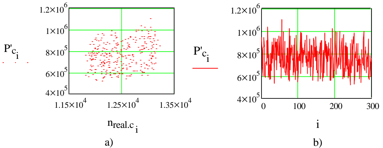
Figure 4.1 Normal measured values of pressure after compressor along different operation regime with accounting measuring errors.
