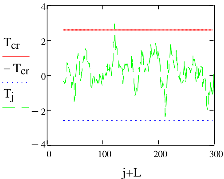
Figure 4.19 Statistic dependence of the Student's distribution with critical boundaries for temperature before working turbine parameter.
