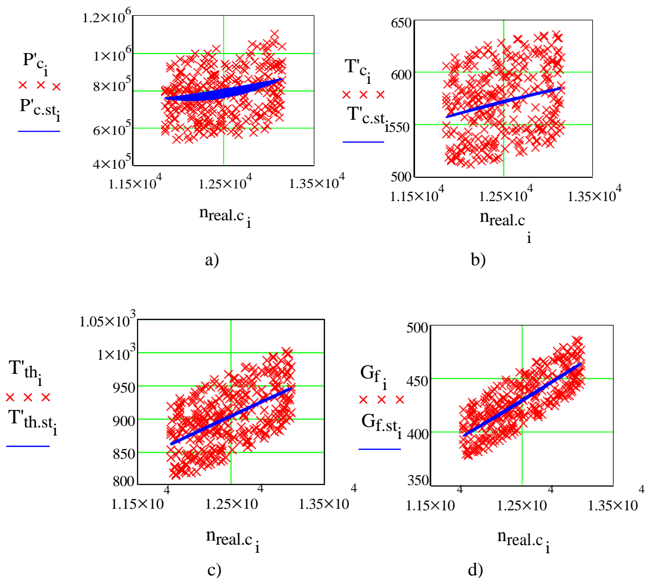
Figure 3.7 – Comparison of measured parameter and ideal parameter for pressure after compressor (a), temperature after compressor (b) and before working turbine (c) and mass flow fuel consumption (d) along the different working power.
