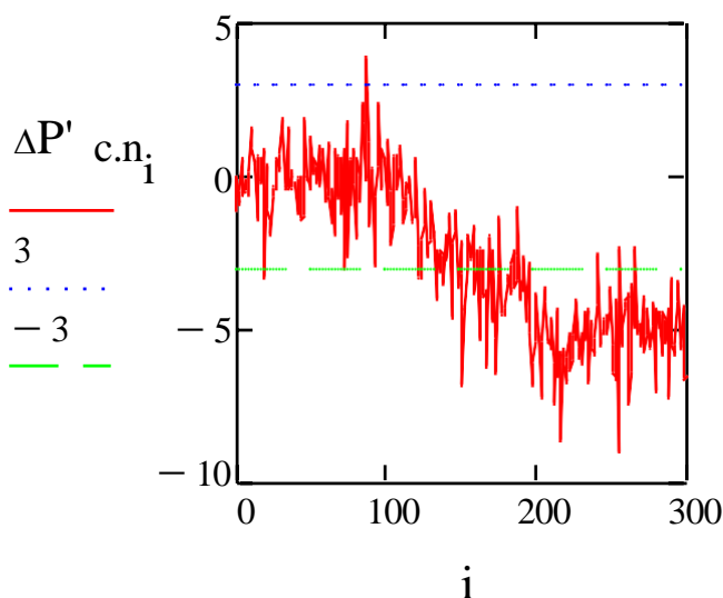
Figure 4.13 Normalized compressor pressure diagnostic deviation dependence from the measurement number.
