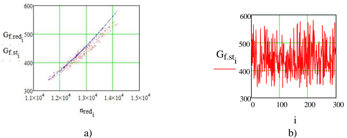
Figure 4.8 Comparison of normal measured mass fuel consumption of GTE and ideal measured parameter ( G_f – normal, G_f – ideal).
