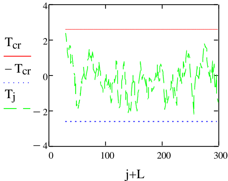
Figure 4.20 Statistic dependence of the Student's distribution with critical boundaries for mass fuel consumption parameter.
