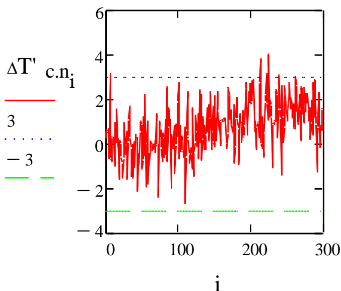
Figure 4.14 Normalized compressor temperature diagnostic deviation dependence from the measurement number.
