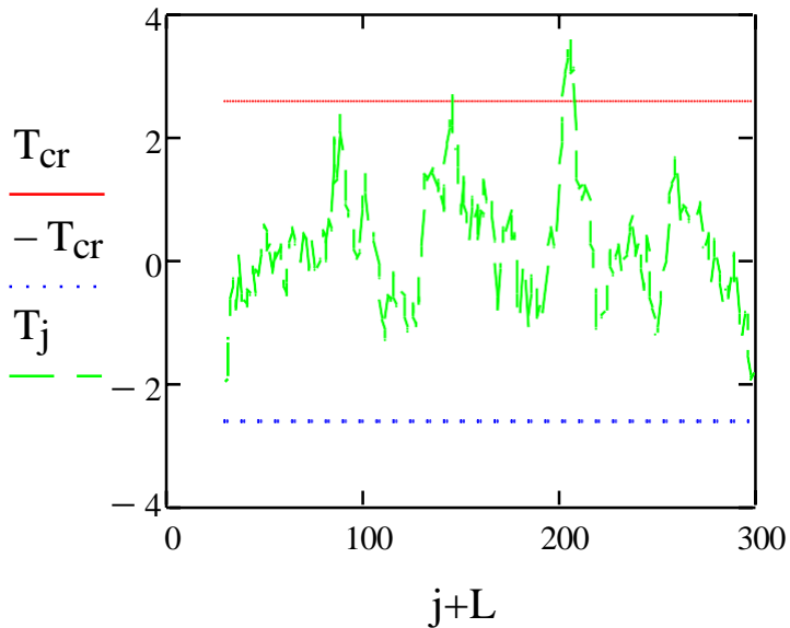
Figure 4.18 Statistic dependence of the Student's distribution with critical boundaries for temperature after compressor parameter.
